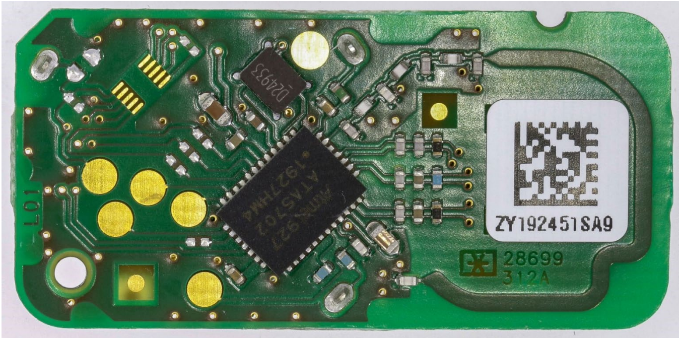
Figure 31: Top.
