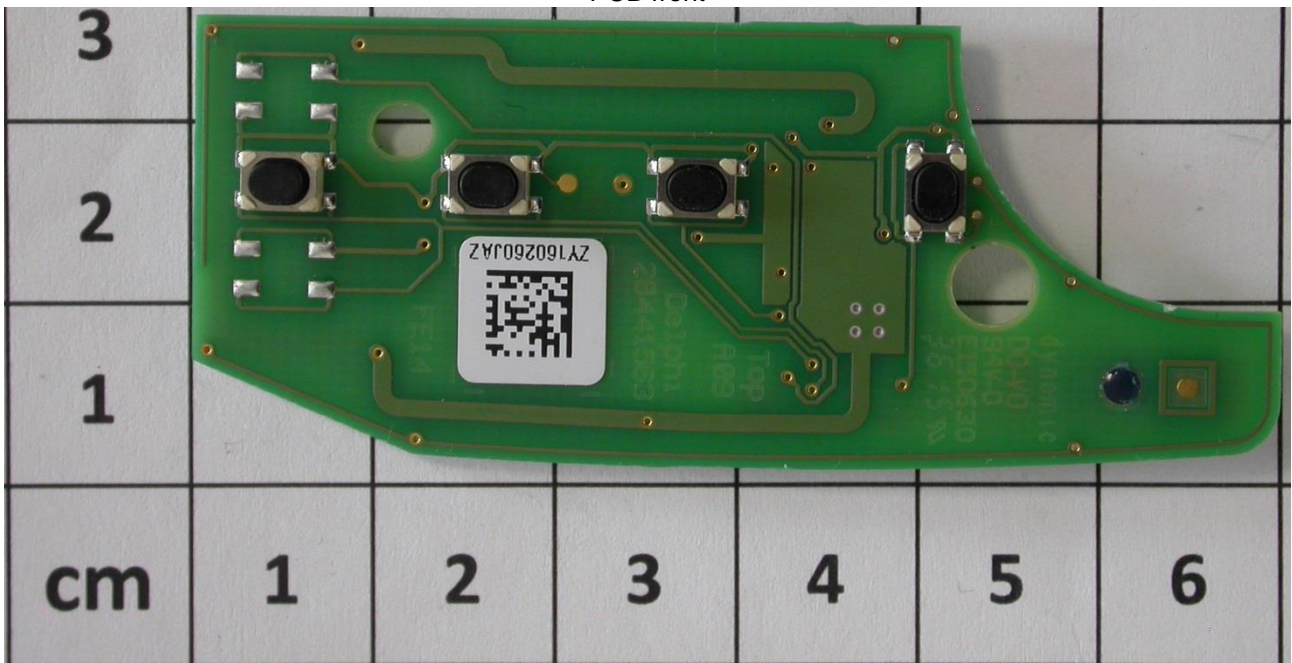
PCB front
