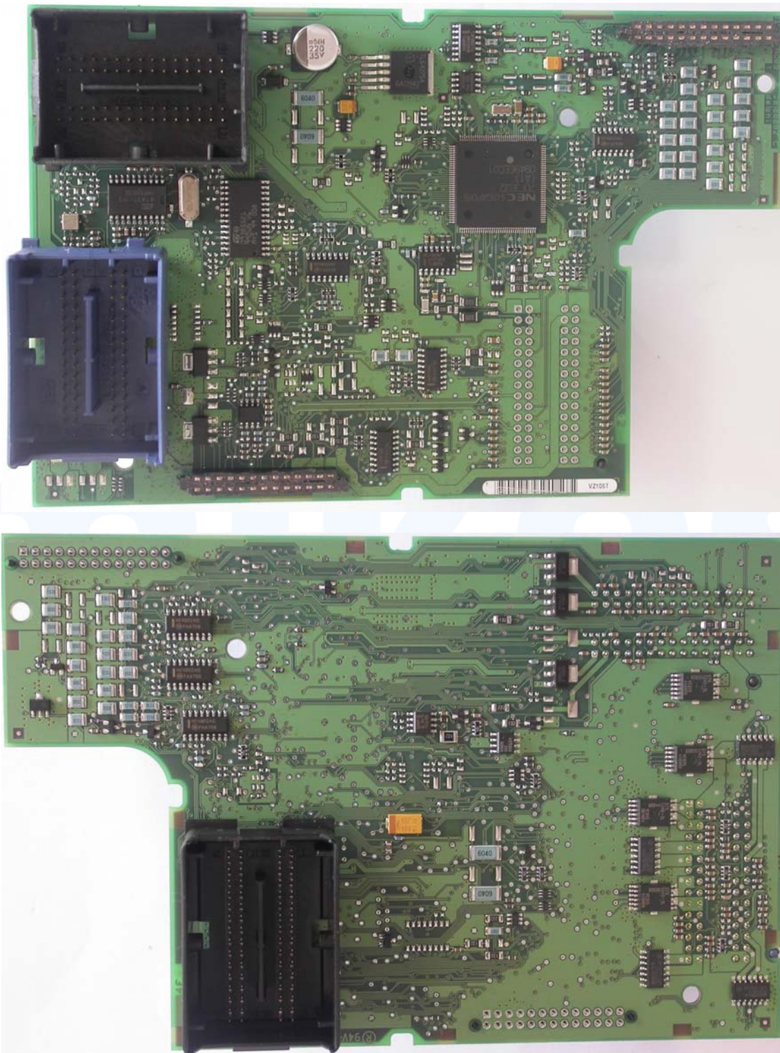
Circuit board 1:
