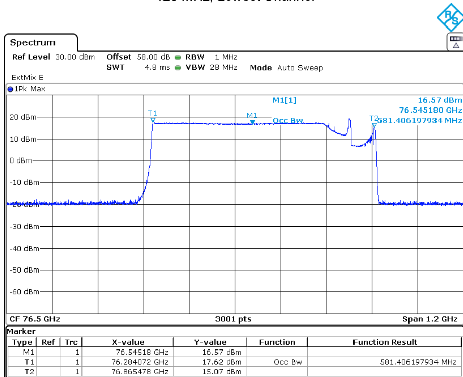
425 MHz, Lowest Channel
