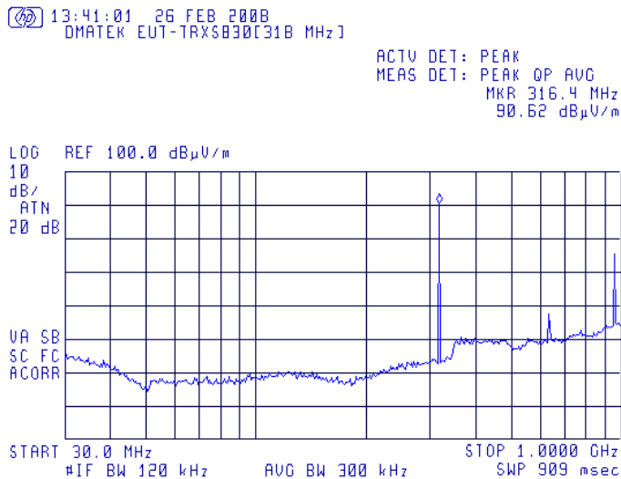
Plot # 2. Spurious emissions scan 30 – 1000 MHz. Test distance =3m.
