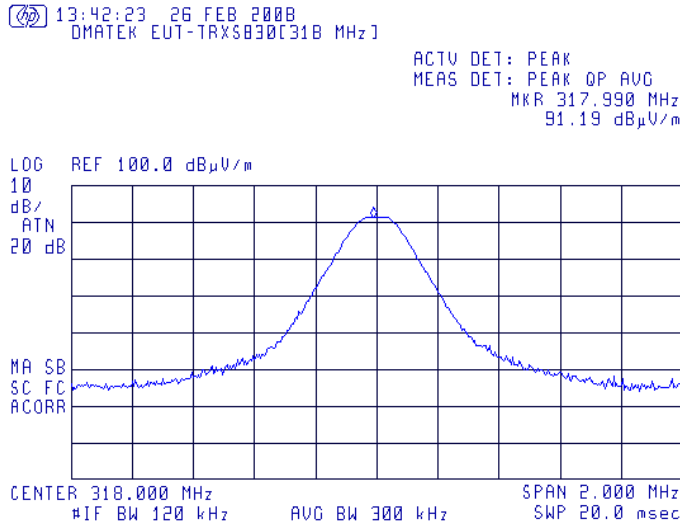
Plot # 1. Field strength of fundamental frequency 318 MHz.
