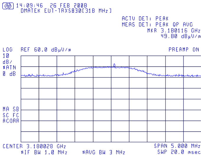
Plot # 9. The carrier frequency 10 th harmonic. Detector peak.
