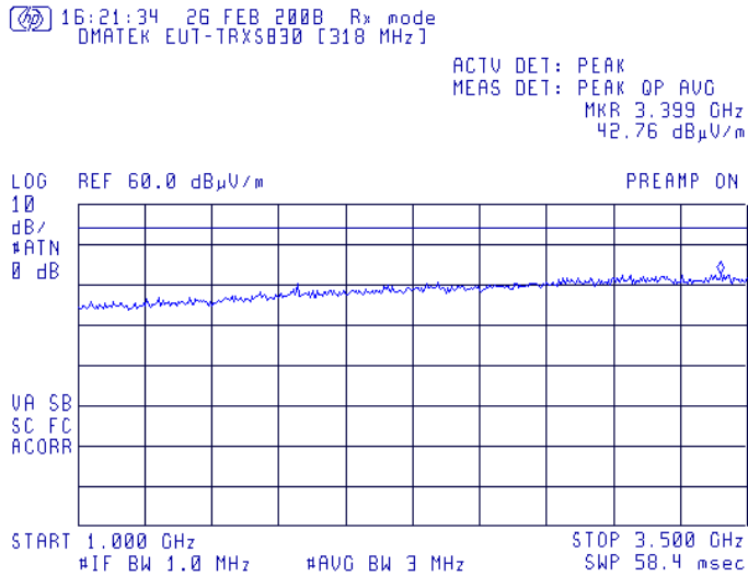
Plot # 11. Rx mode. Scan of spurious emissions. Frequency range from 1 GHz to 3.5 GHz. Test distance =3m
