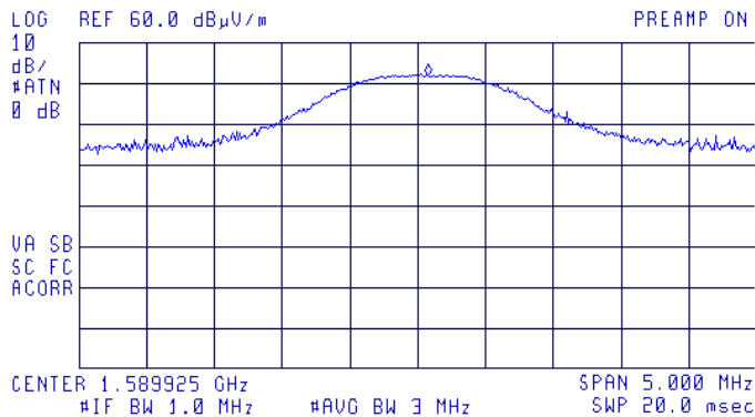
Plot # 6. The carrier frequency 5 th harmonic. Detector peak.
