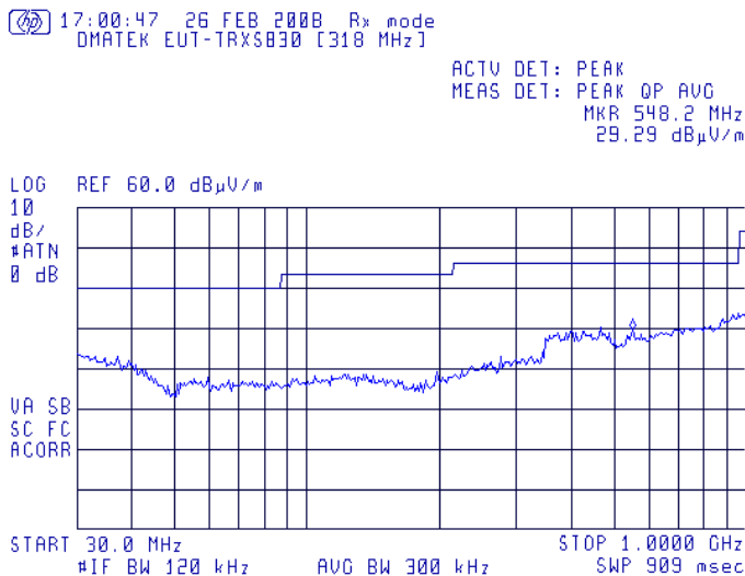
Plot # 10. Rx mode. Scan of spurious emissions Frequency range from 30 MHz to 1000 MHz. Test distance =3m.
