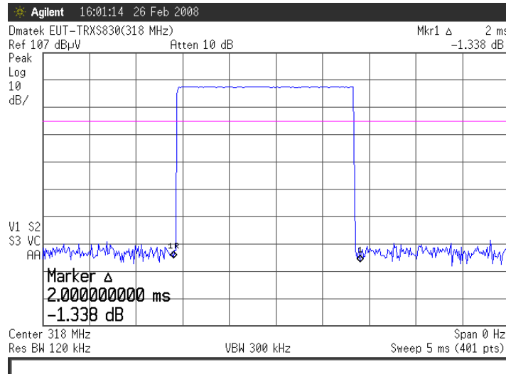
Plot # 12. Transmission duration - Tx on.
