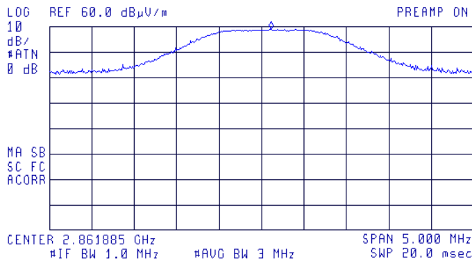
Plot # 8. The carrier frequency 9 th harmonic. Detector peak.
