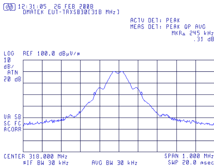
Plot # 14. Occupied bandwidth test result
