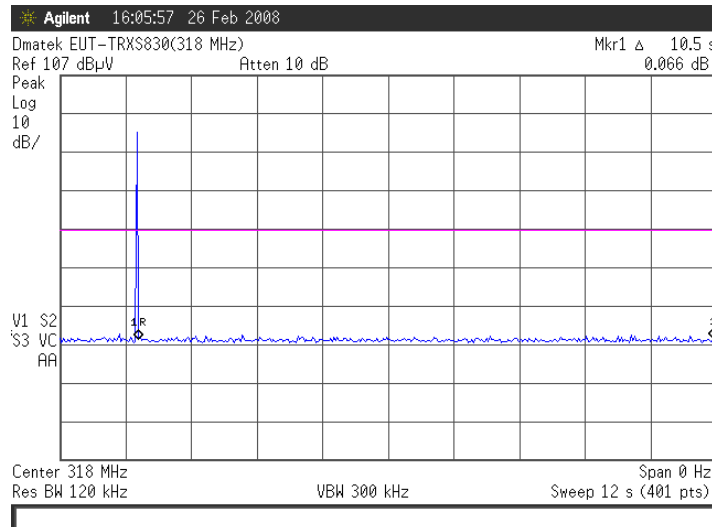
Plot # 13. Transmission duration - Tx off
