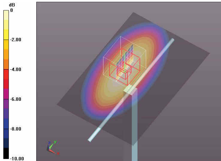
0 dB = 3.12 W/kg = 4.94 dBW/kg
