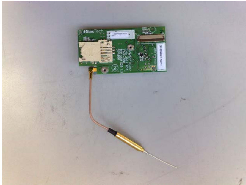
Figure 6: Cellular Module and Antenna (Bottom)
