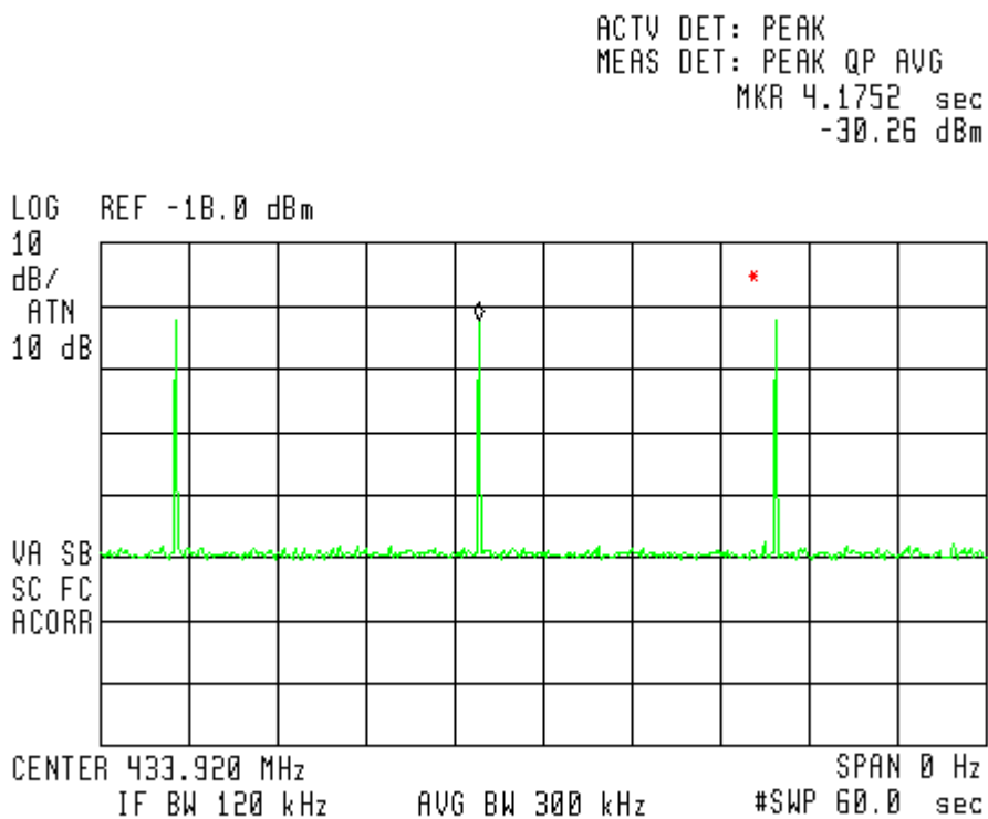
Figure 10. System Integrity Every Minimum 20 sec
