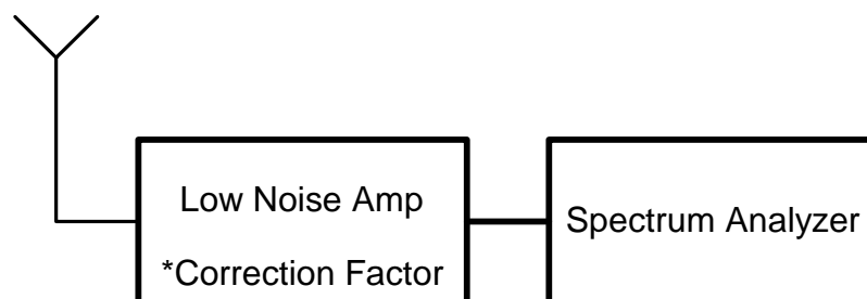
Figure- 2 Radiated Emission test 9KHz – 10GHz
