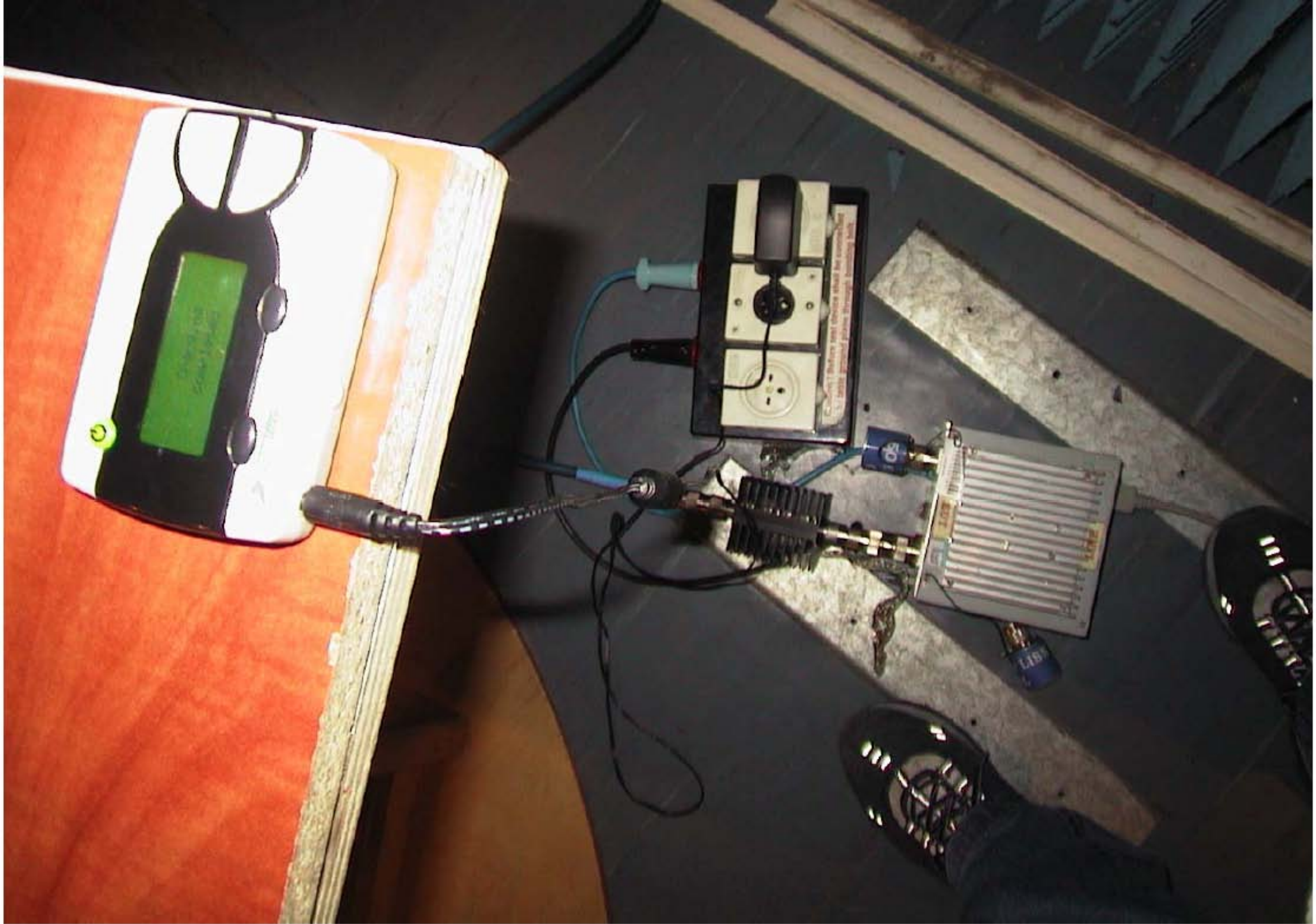
Conducted emission Test Set up
