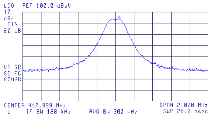
Plot # 1. Field strength of fundamental frequency 418 MHz.
