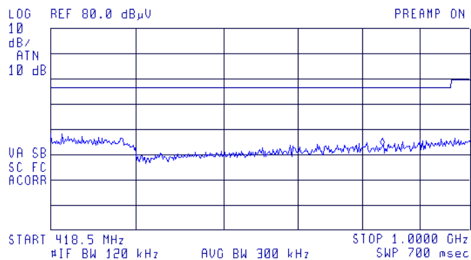
Plot # 4. Spurious emissions scan 418.5 MHz – 1000 MHz.
