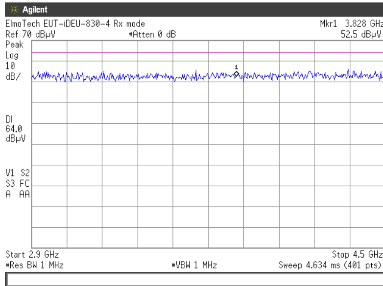
Plot # 10. Scan of spurious emissions in receive mode. Frequency range from 2.9 GHz to 4.5 GHz.
