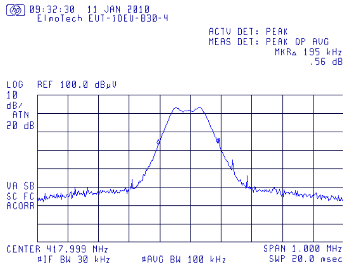
Plot # 12. Occupied bandwidth test result
