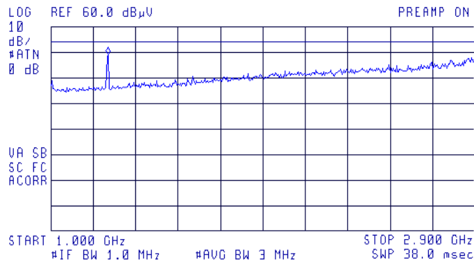
Plot # 5. Spurious emissions scan at 1.0 – 2.9 GHz frequency range.
