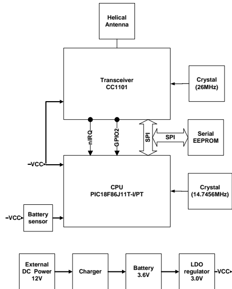
Figure 1. Repeater block diagram.
