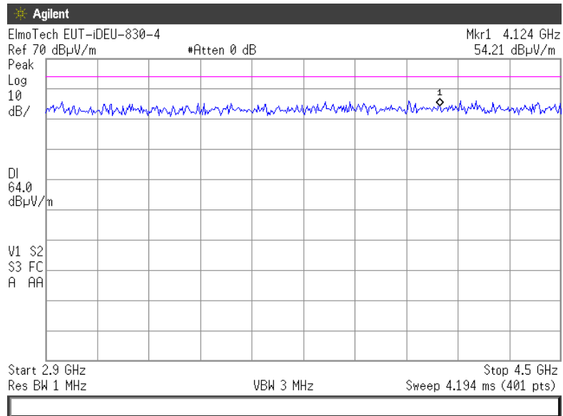
Plot # 7. Spurious emissions scan at 2.9 – 4.5 GHz frequency range.
