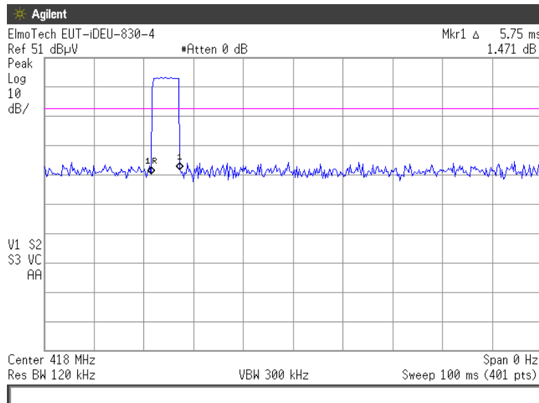
Plot # 11. Transmission duration - Tx on.
