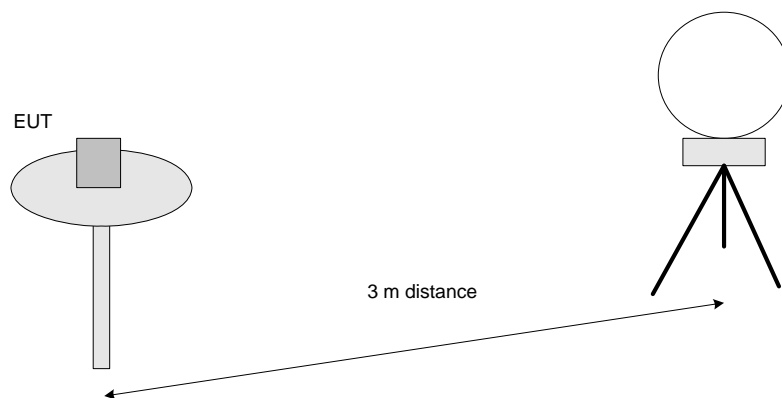
Figure 2. Radiated emission test setup diagram.
