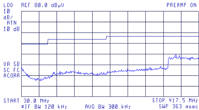
Plot # 3. Spurious emissions scan 30 – 417.5 MHz. Test distance 3m.
