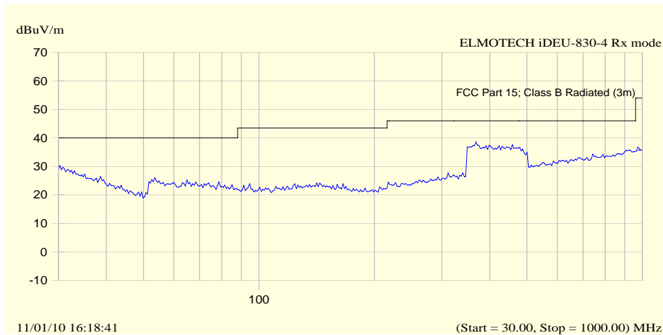
Plot # 8. Radiated emission test in receive mode. Frequency range from 30 MHz to 1000 MHz.
