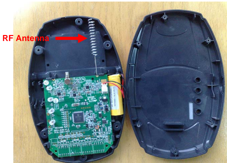
Figure 1: IDEU-830-4 (Open)
