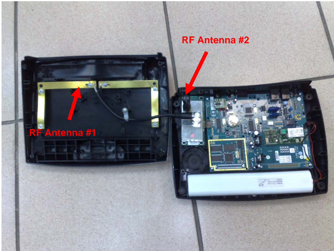
Figure 1: DCU-2010-2 (Open)
