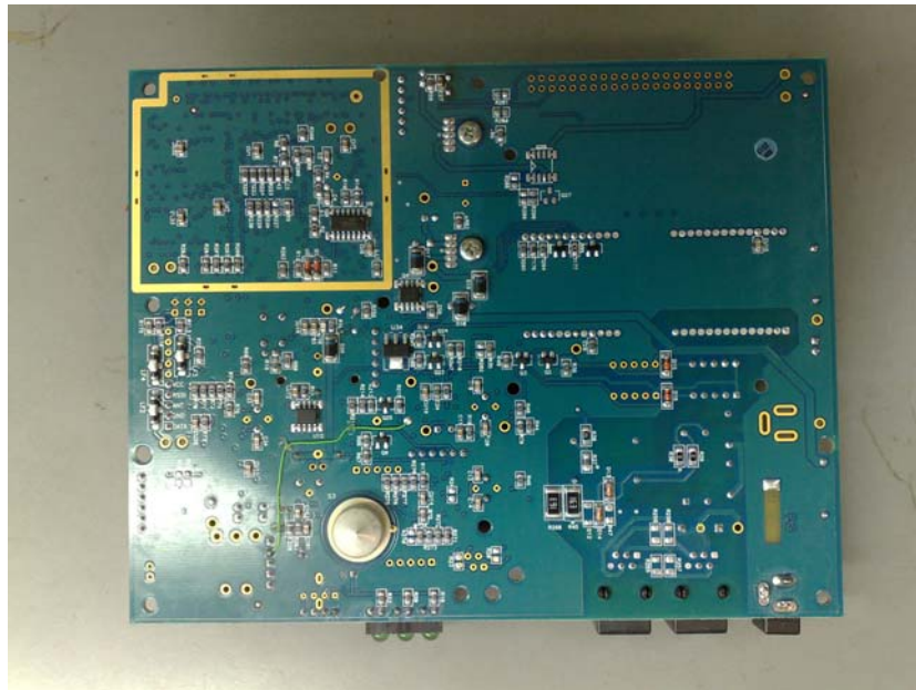
Figure 4: Main Board (Bottom)
