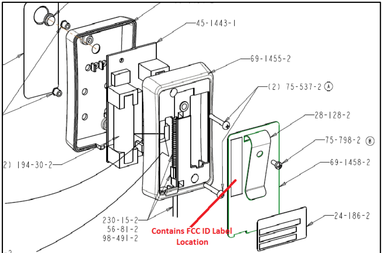
Photograph 3: "Contains FCC ID:...." Label Location on Back of Sample Host
