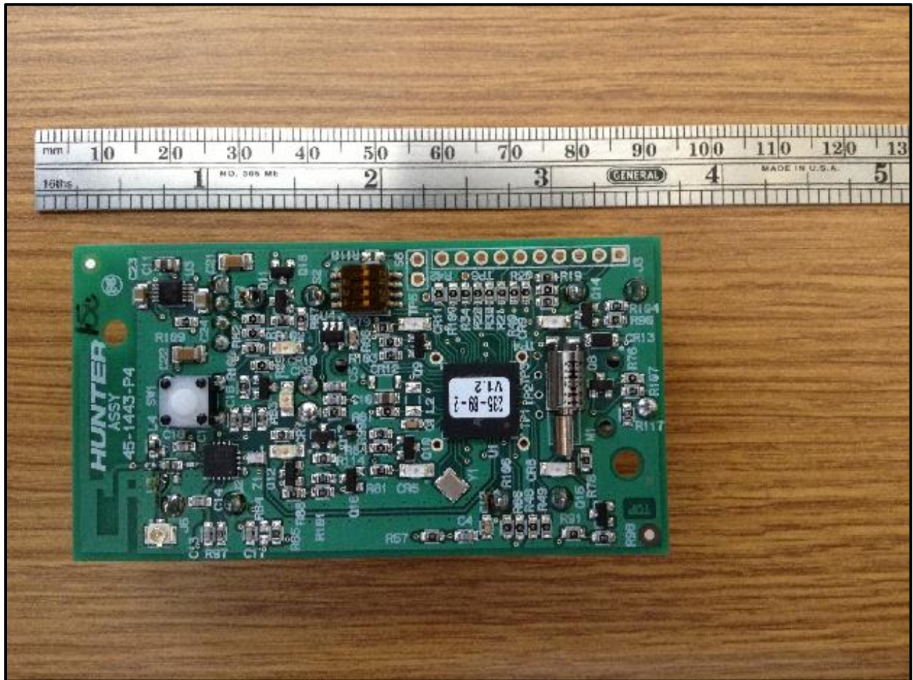
Photograph 13: PCB Front without Shield
