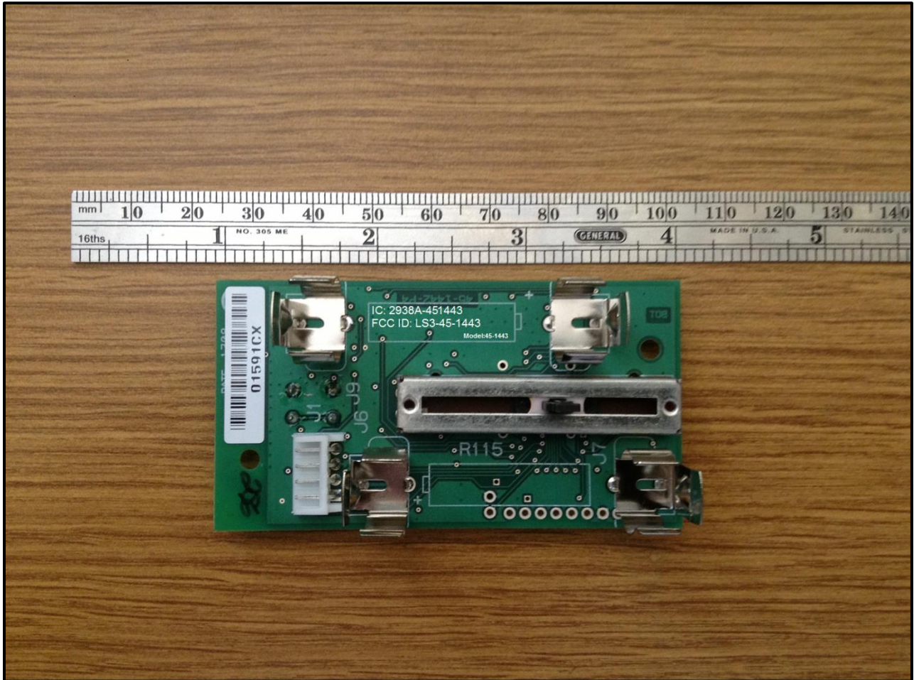
Photograph 14: PCB Back
