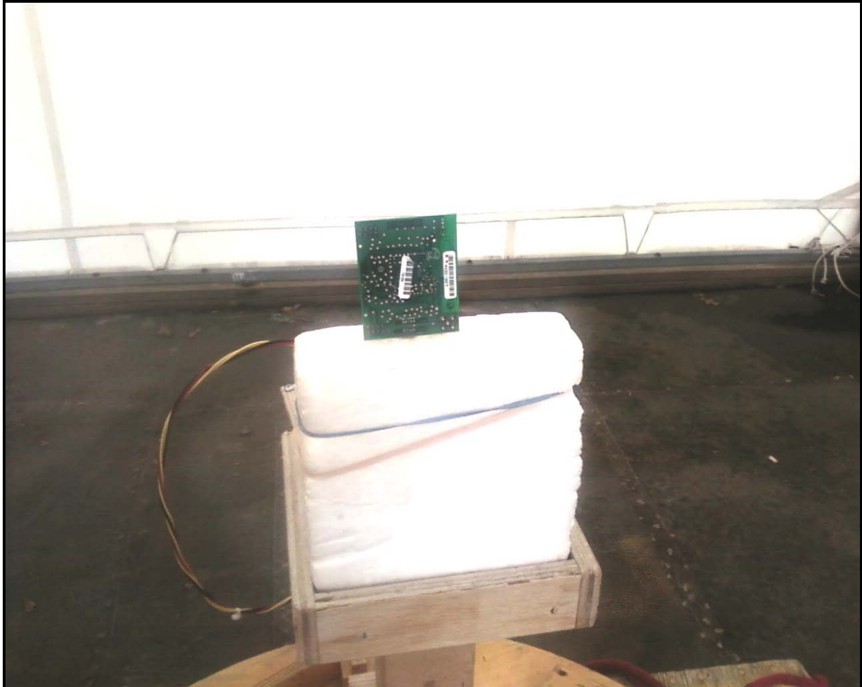
Photograph 4: Radiated Emissions Testing – Back View
