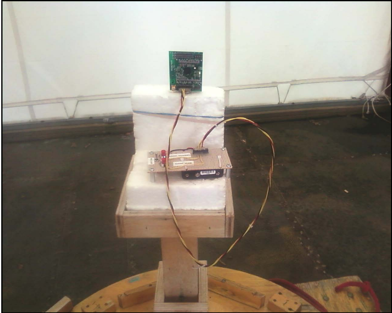
Photograph 3: Radiated Emissions Testing – Front View
