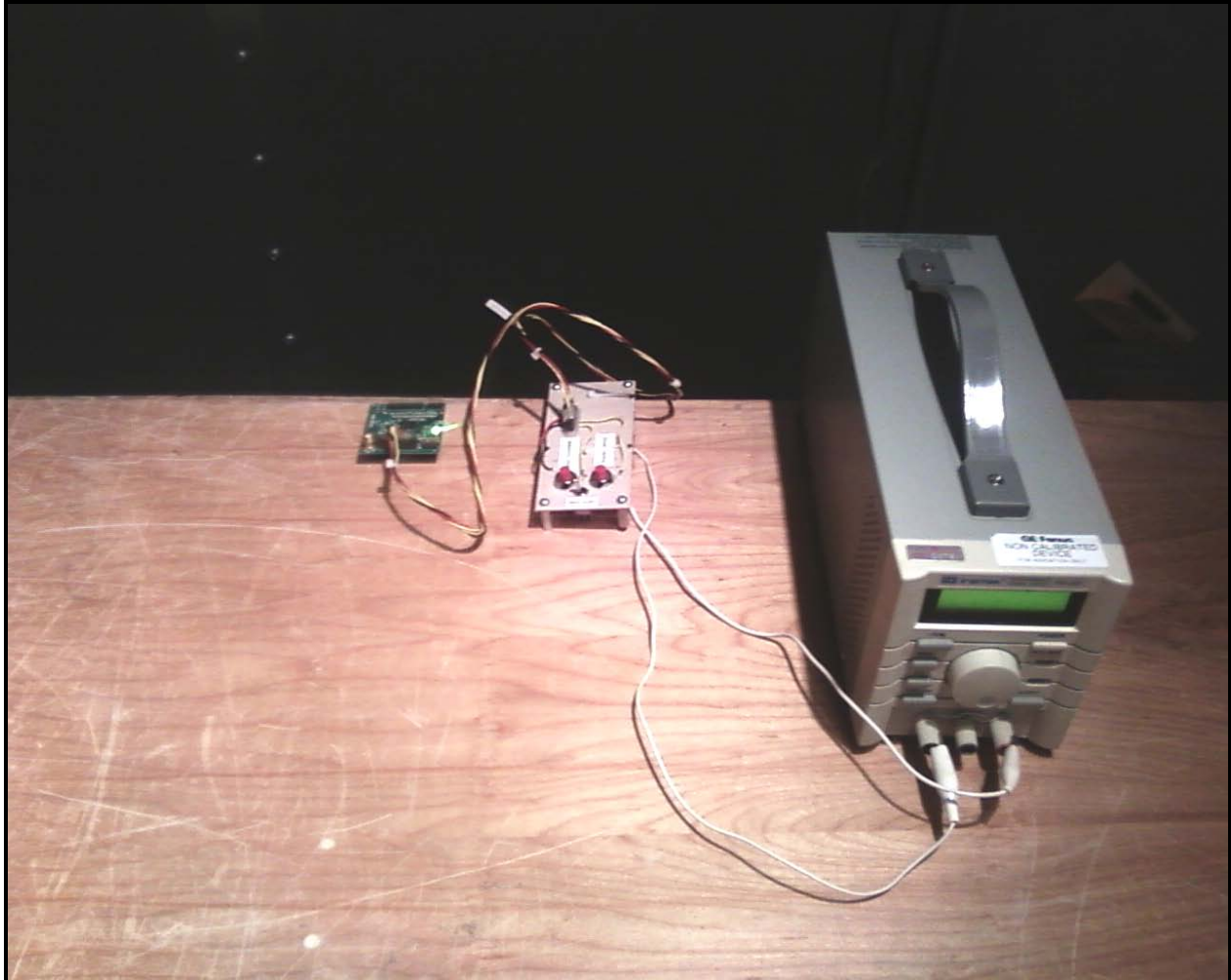
Photograph 5: Conducted Emissions Testing – Front View
