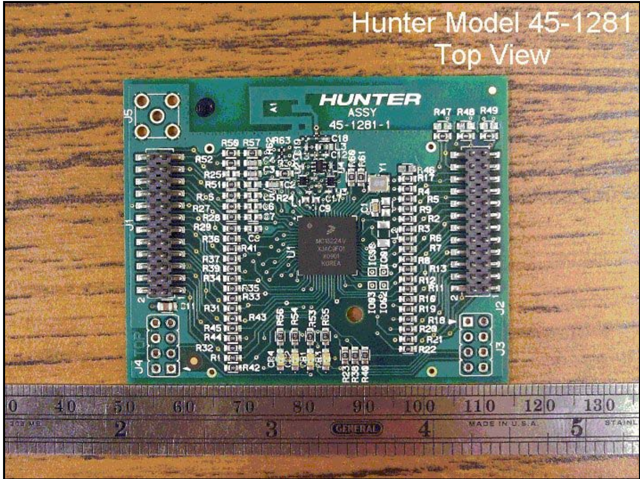
Photograph 11: Top of PCB without Shield
