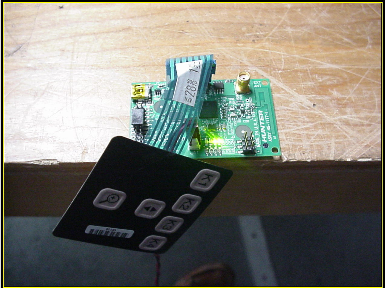
Photograph 6: Conducted Emissions Testing – Back View
