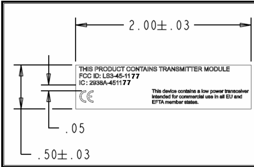
Photograph 2: "Contains FCC ID....." Label Sample
