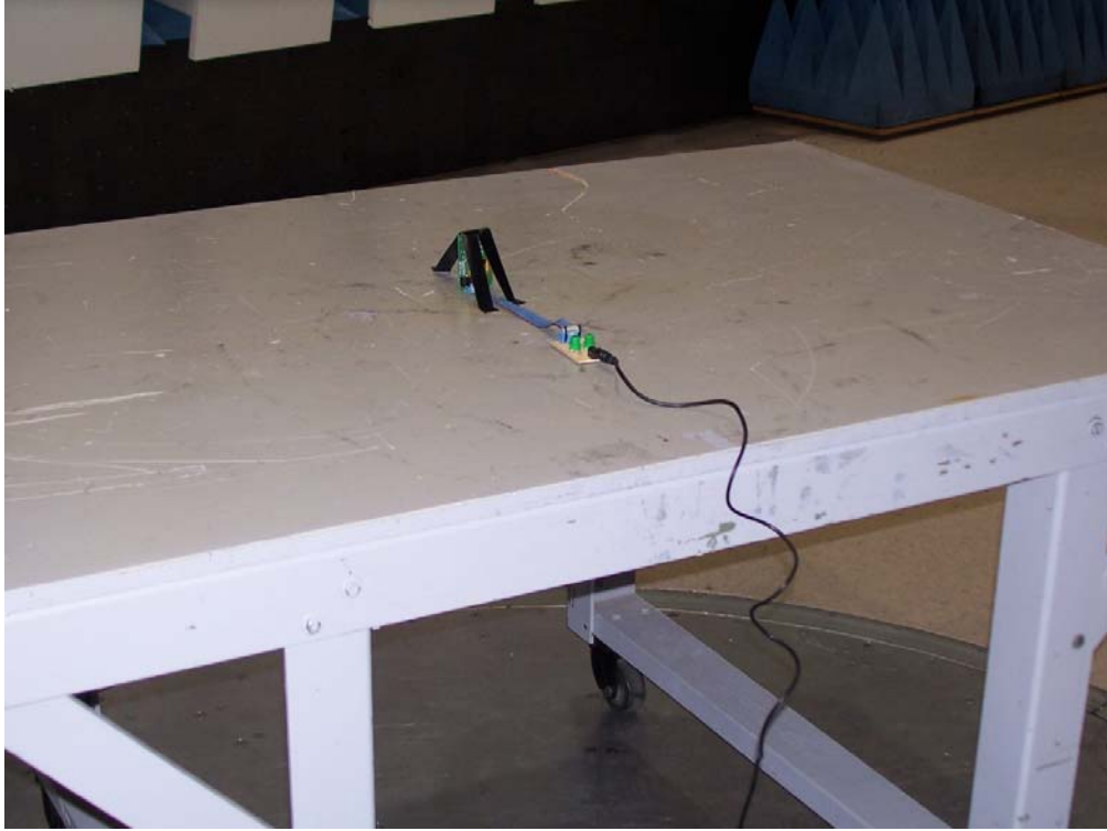
Figure 2 - Radiated Emissions, Band Edge Compliance, and Voltage Variations vs. Frequency Stability Test Setup Test Setup (Chamber - Back)
