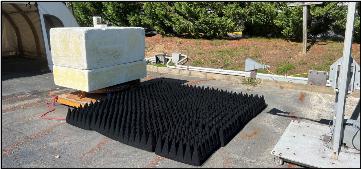
Photograph 4: Radiated Emissions Testing – Back View (> 1 GHz)
