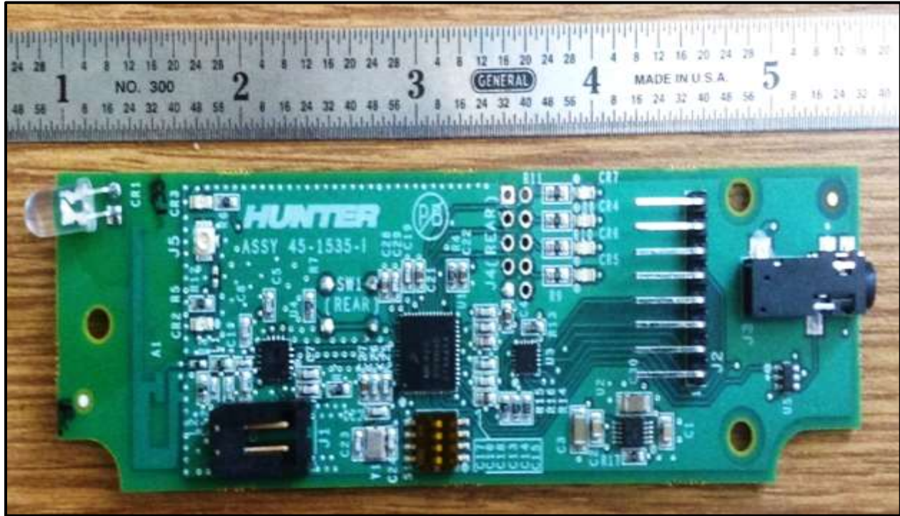
Photograph 6: PCB Front
