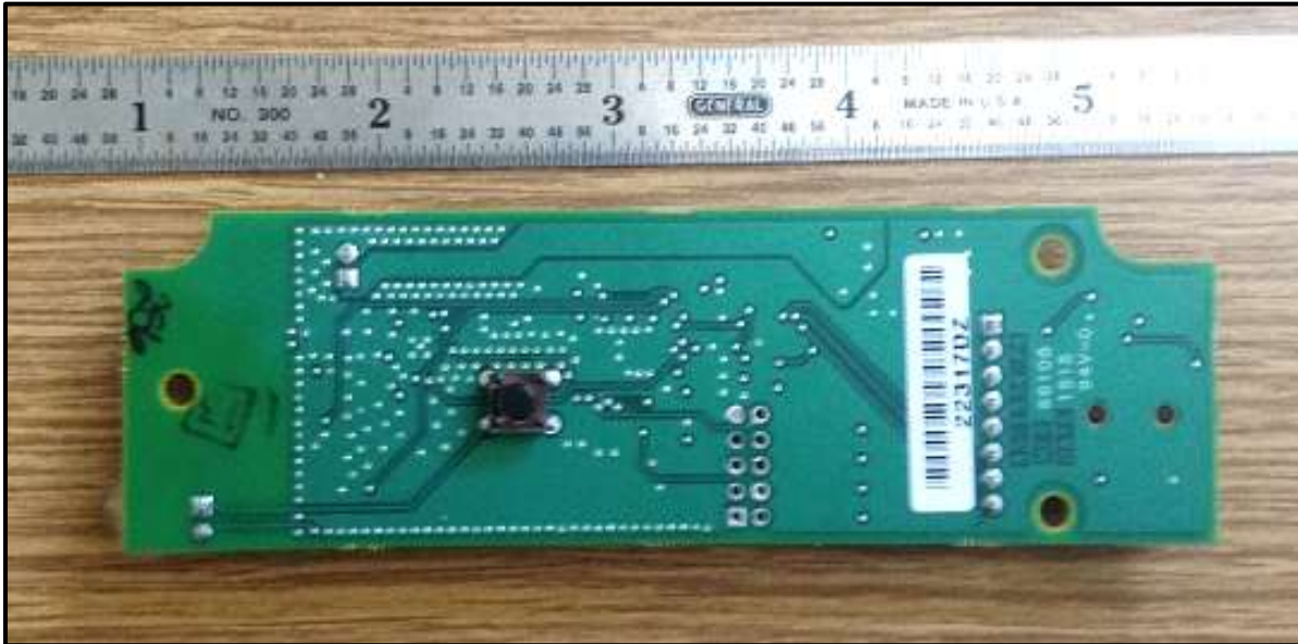
Photograph 7: PCB Back
