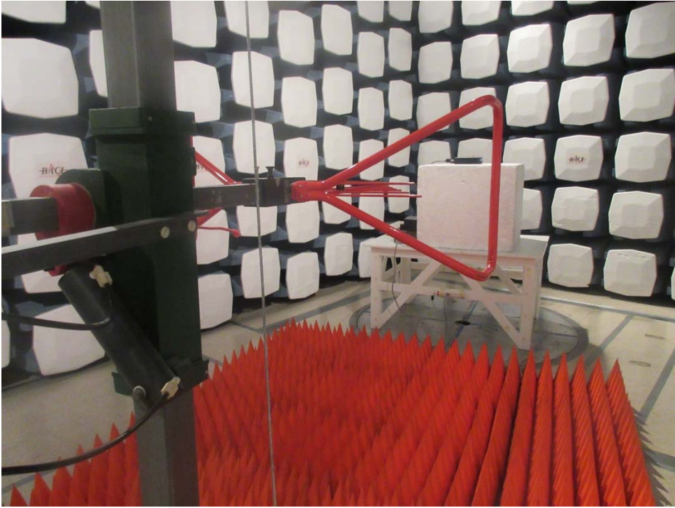
Radiated Emission below 1 GHz (SVR-300V) – Rear View
