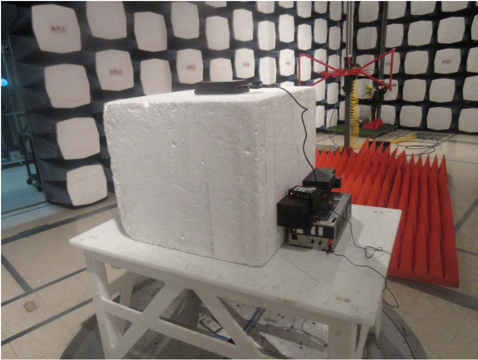
Radiated Emission below 1 GHz (SVR-300V) – Front View
