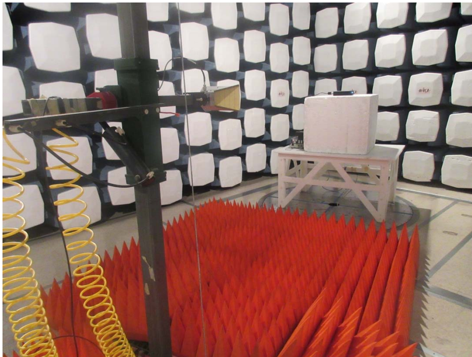
Radiated Emission above 1GHz (SVR-300V) – Rear View
