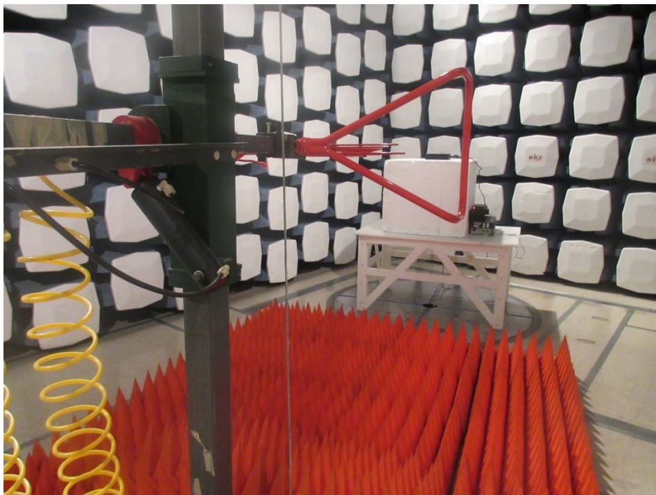
Radiated Emission below 1 GHz (SVR-300UA) – Rear View
