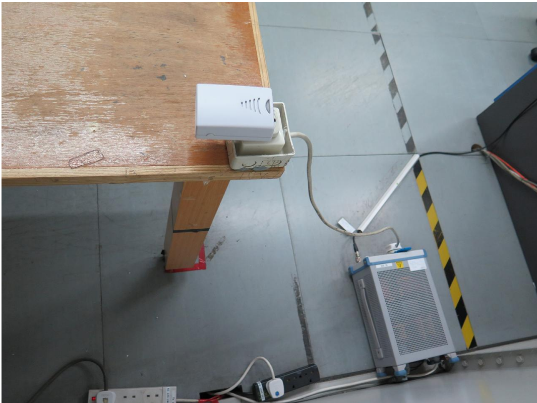
Rear view (Conducted emission)
