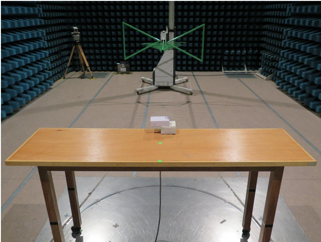
Front view (Radiated emission)
