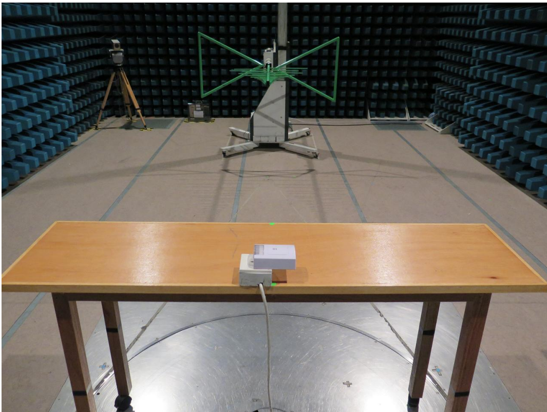
Rear view (Radiated emission)
