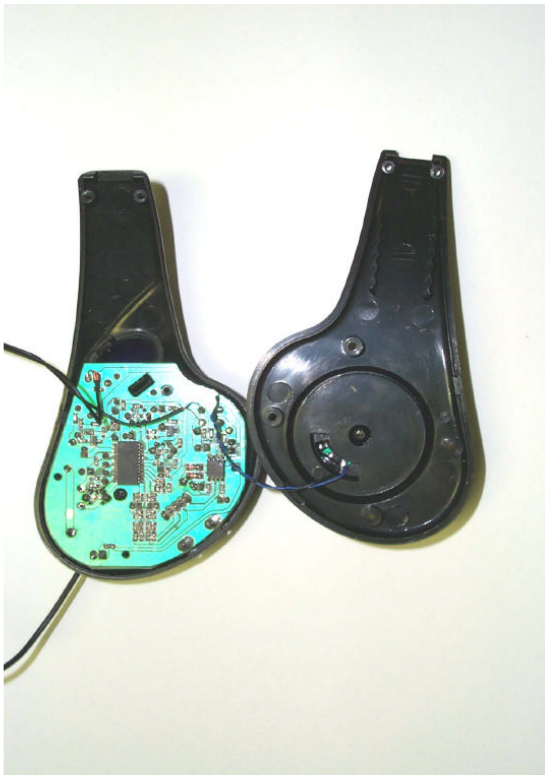
Figure 6.3 Right Side Open view
