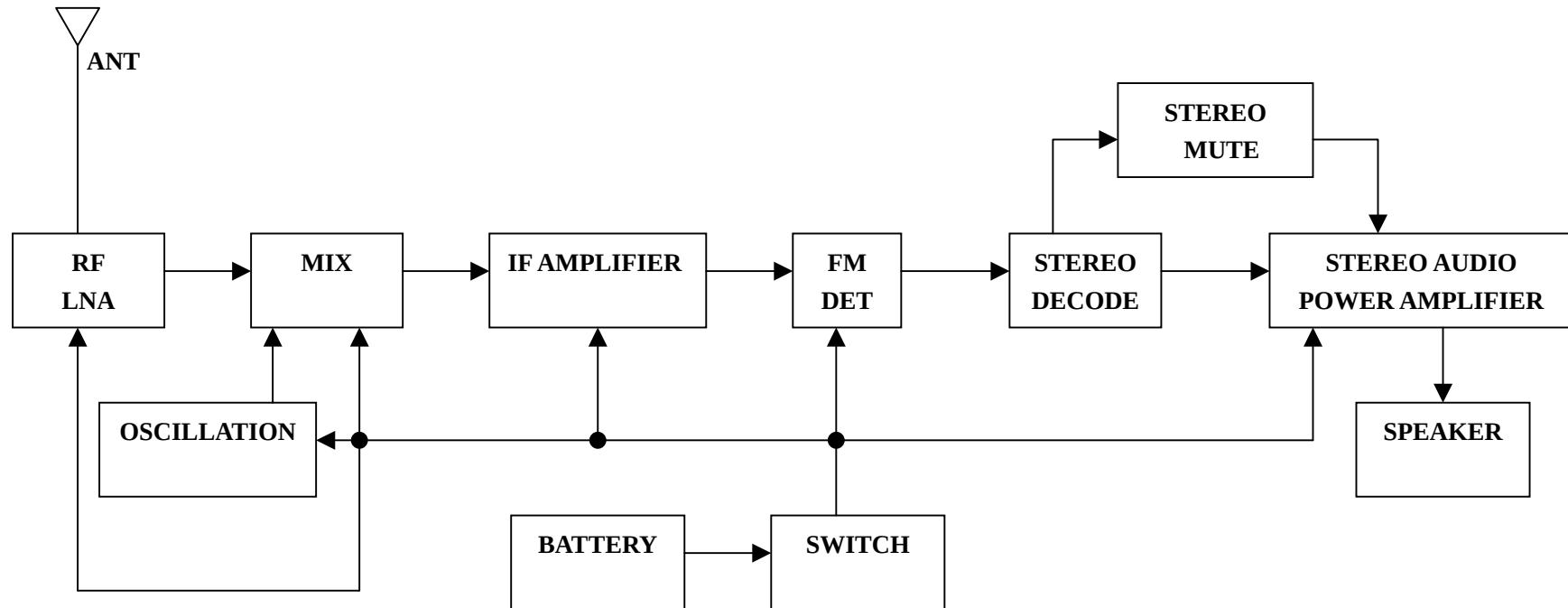
SRF2010 Receiver Block Diagram
