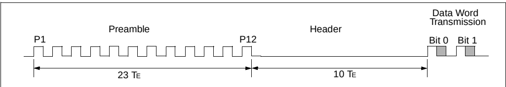
FIGURE 8-3: PREAMBLE/HEADER FORMAT
