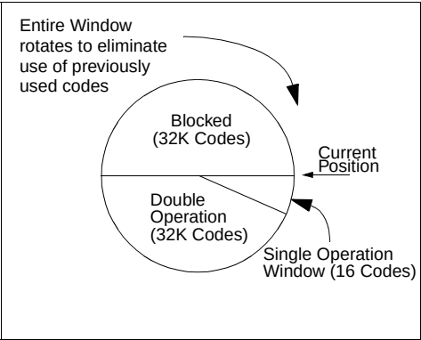
FIGURE 7-3: SYNCHRONIZATION WINDOW
