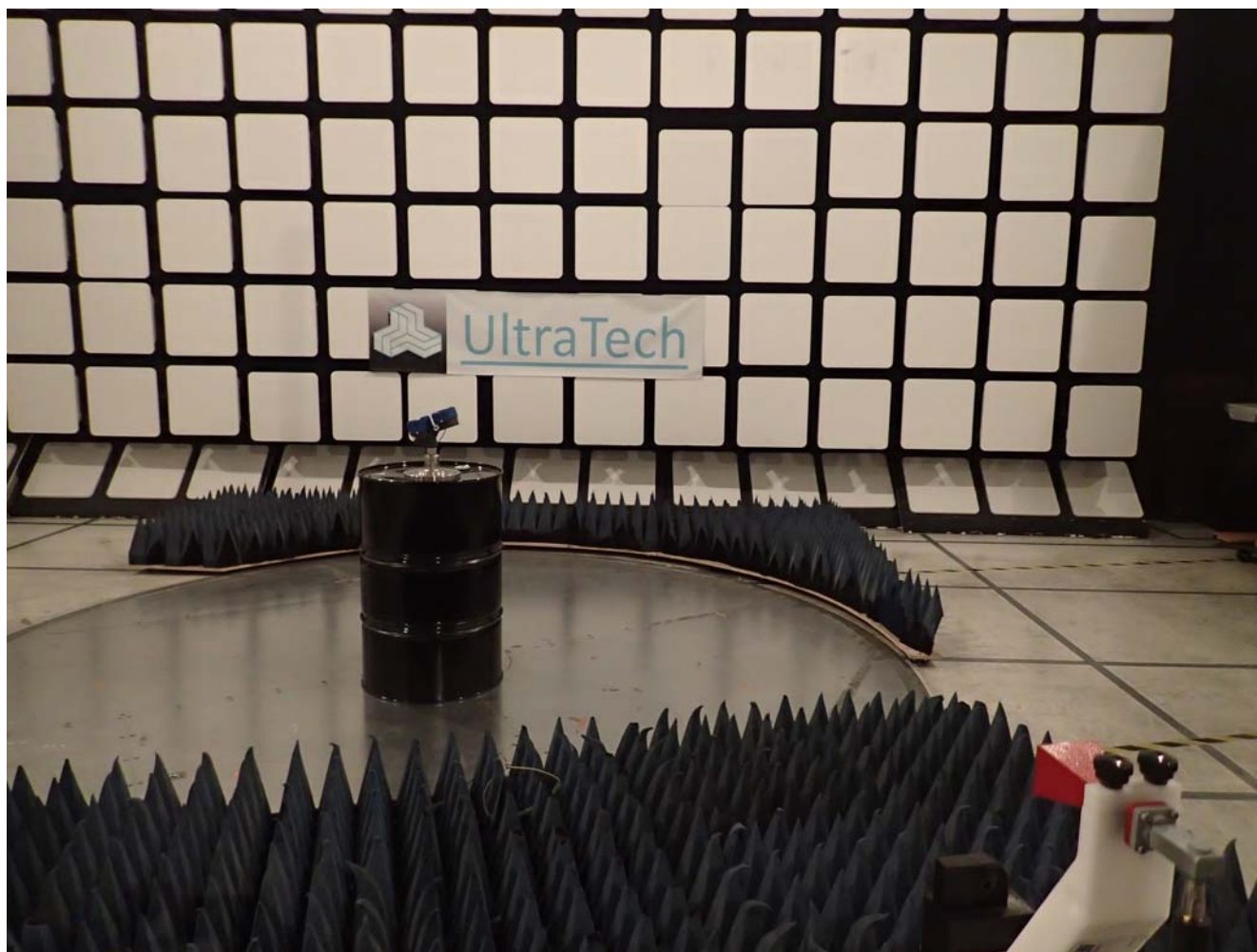
TLPR Radiated Emissions at 3 m Distance (above 1 GHz)
