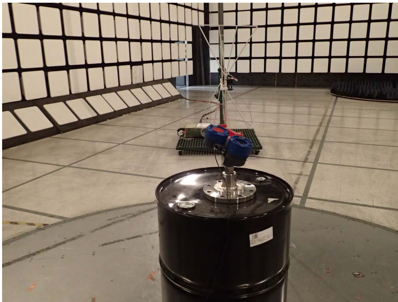
TLPR Radiated Emissions at 3 m Distance (30 - 1000 MHz)
