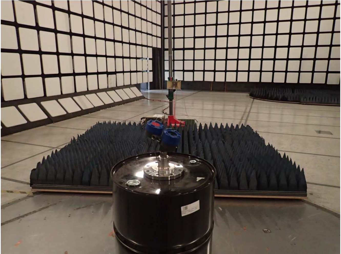
TLPR Emissions at 3 m Distance (above 1 GHz)
