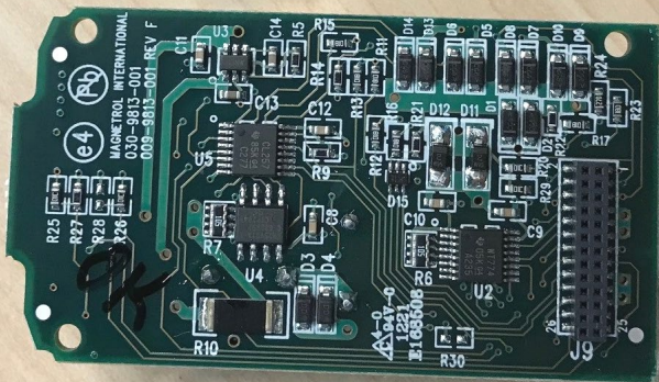
Analog board Bottom
