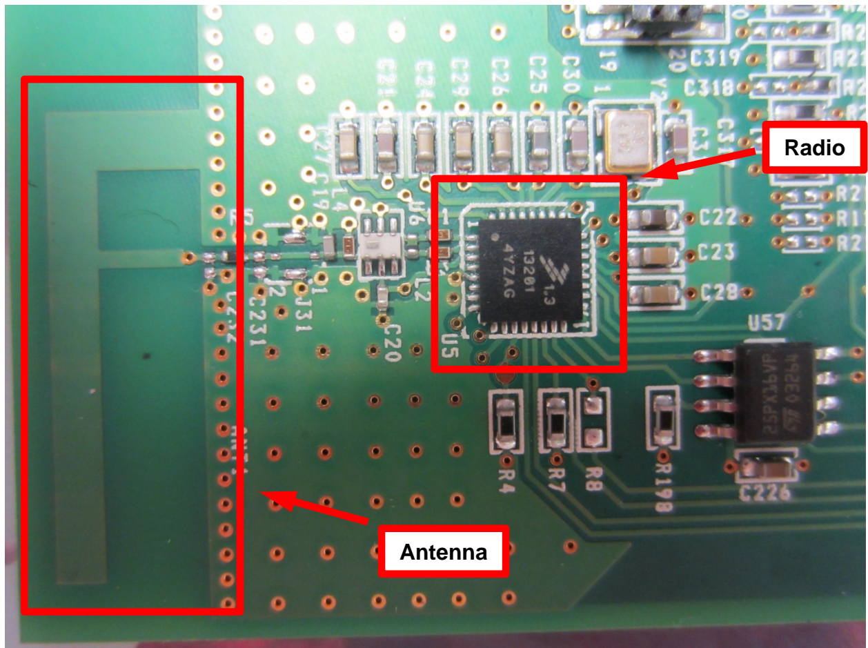
Figure 4 - Detail of antenna and radio on top side of board.
