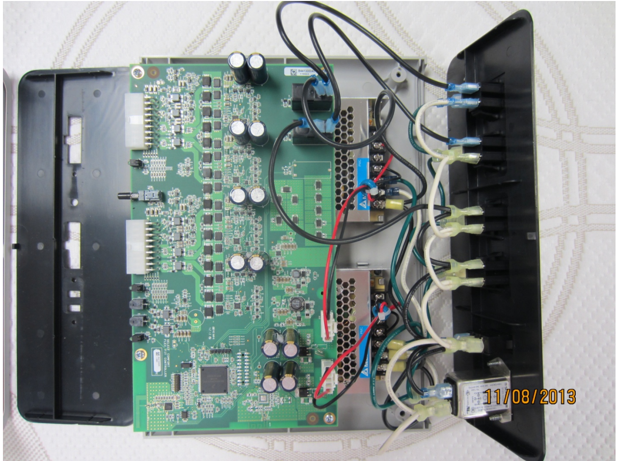
Figure 2 - Assembly Components Top View (2)
