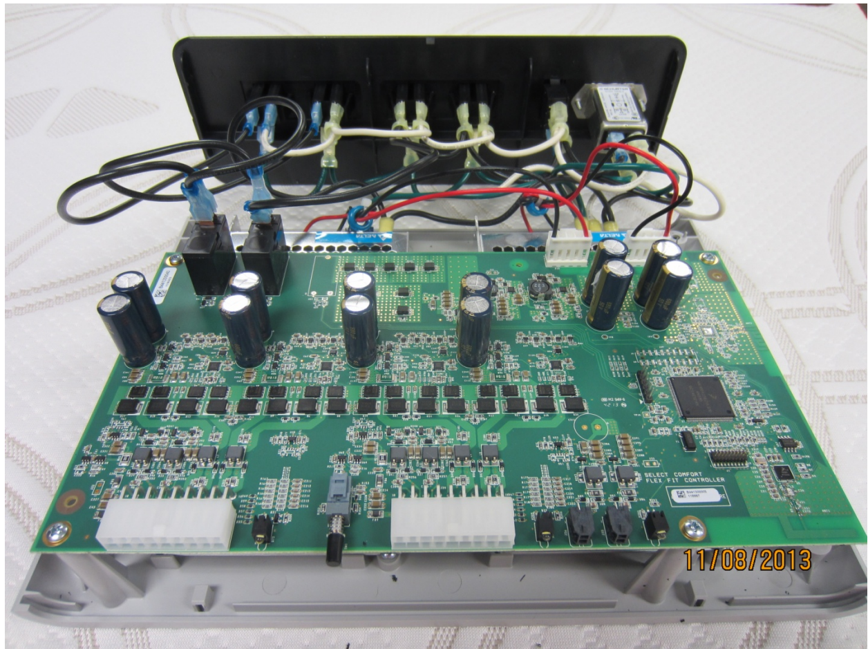
Figure 3 - Assembly Components Top View (3)
