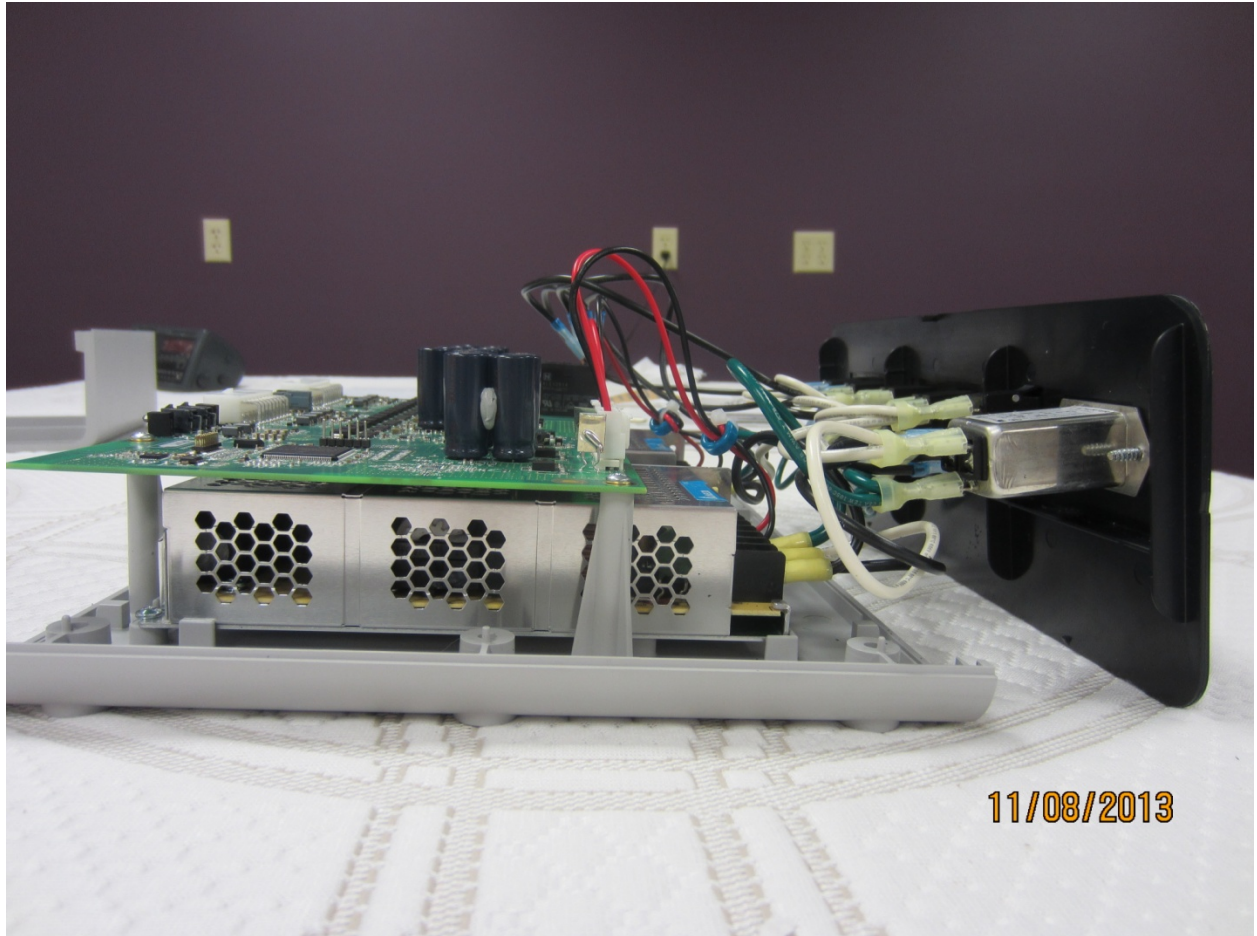
Figure 6 - Assembly Components Side View (3)
