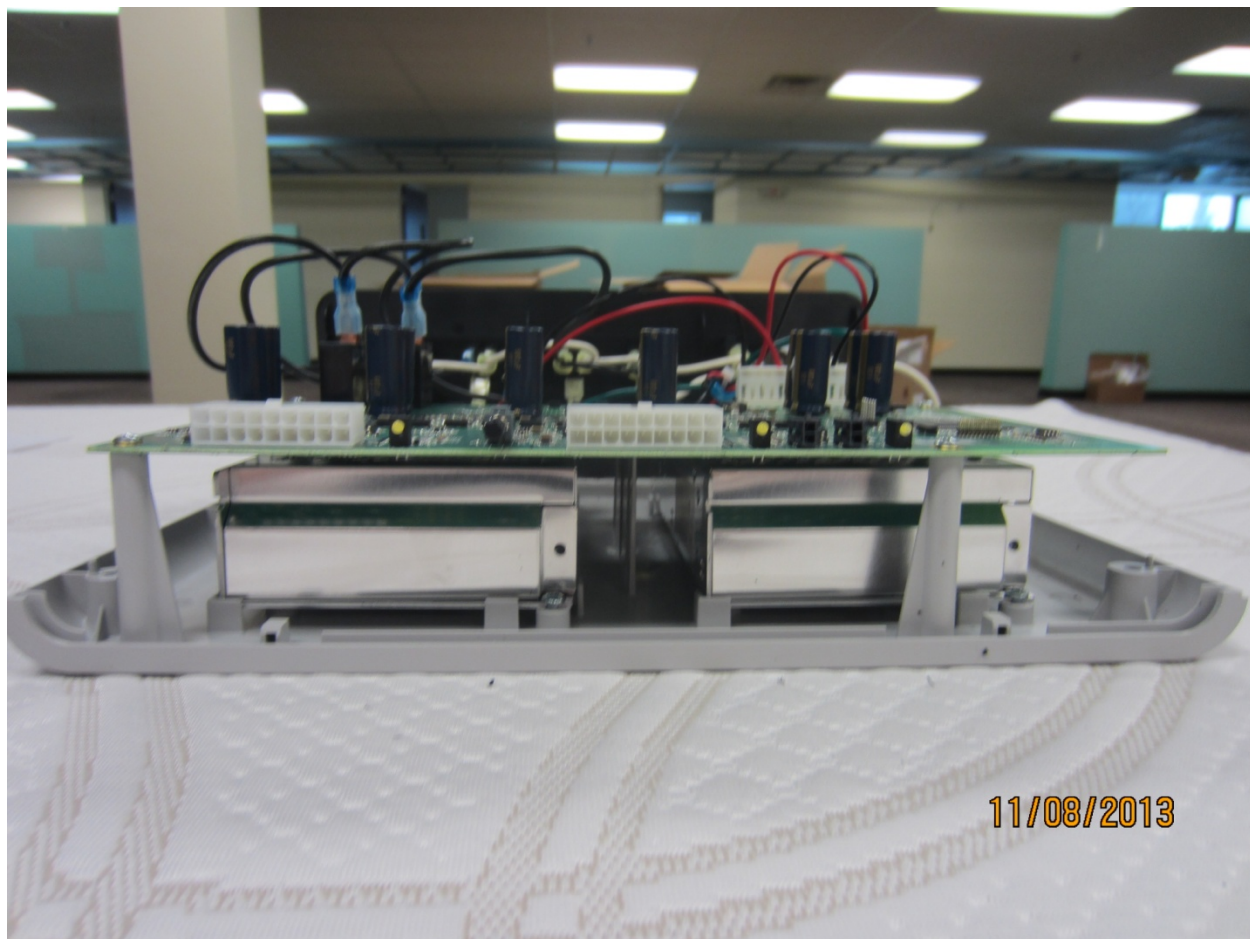
Figure 5 - Assembly Components Side View (2)
