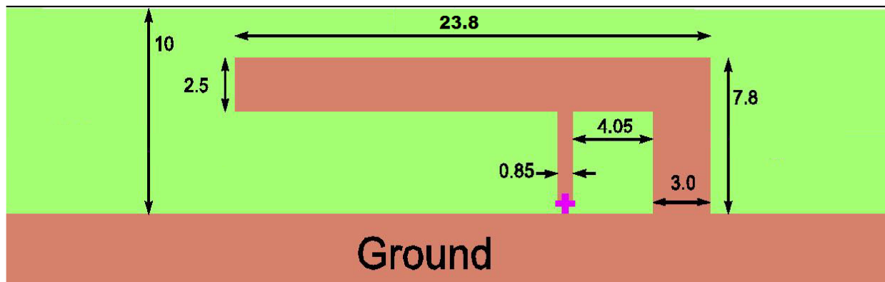
Figure 4. F Antenna
