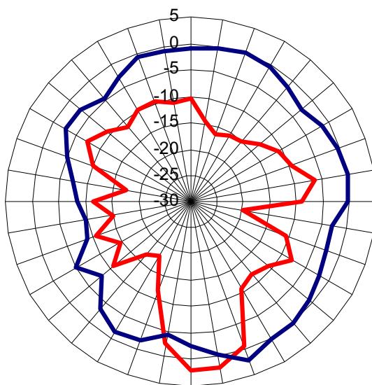
Figure 5. F-Antenna Radiation Pattern (For Antenna as Shown in Figure 11)
