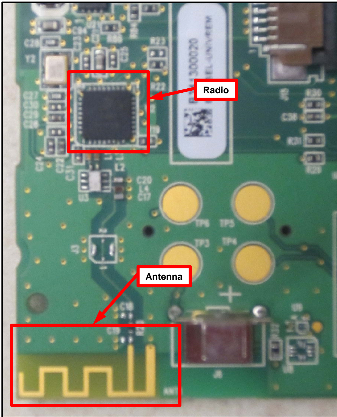
Figure 3 - Detail of antenna and radio on rear side of board.
