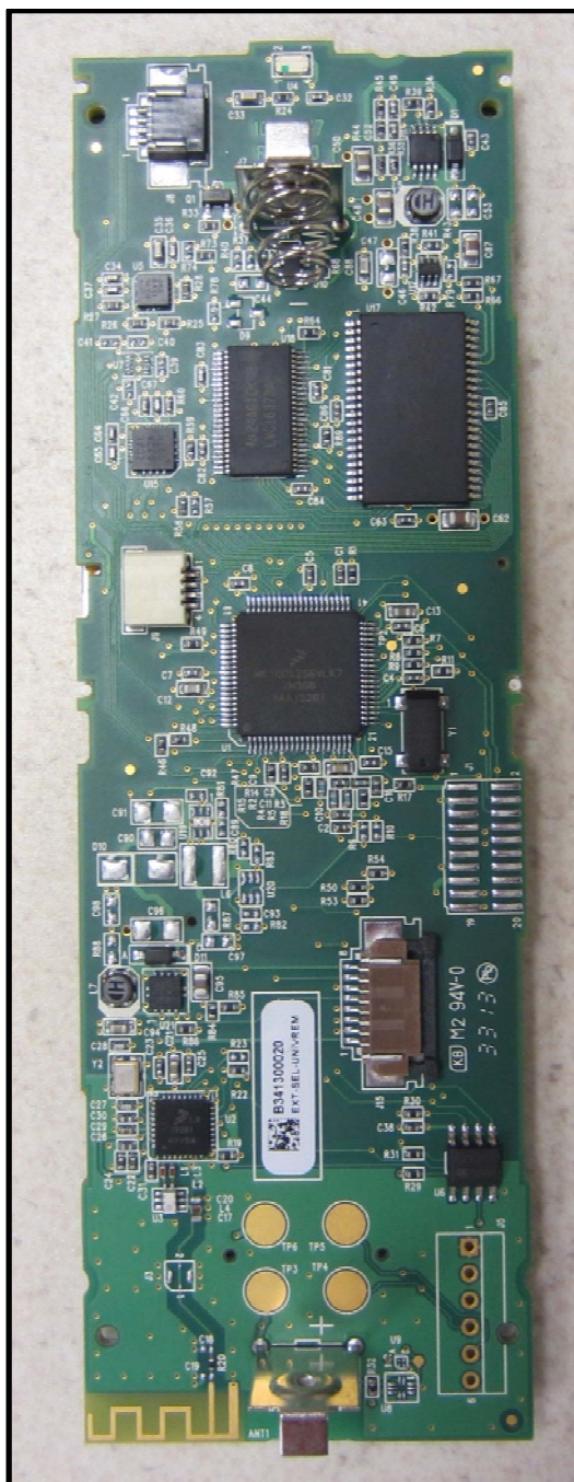
Figure 1 – Rear Side of Circuit Board
