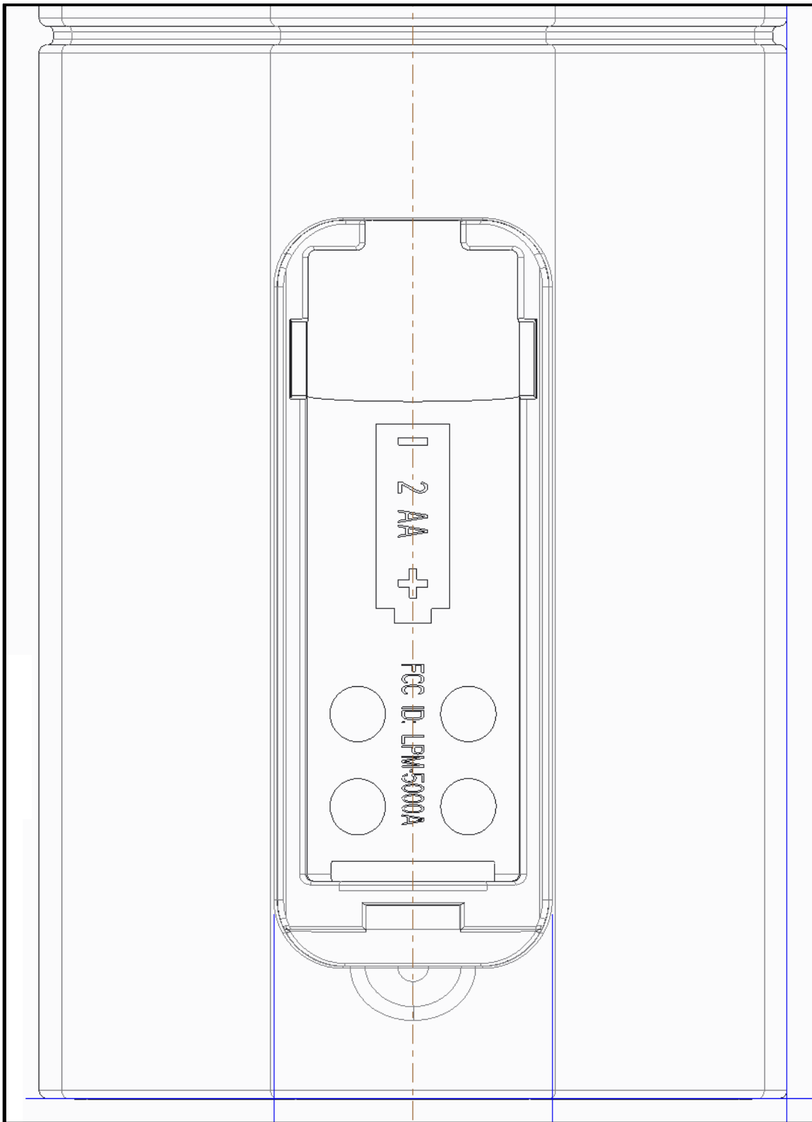
Figure 2 - Detail from case drawing showing location where FCC ID will be molded into the battery compartment.
