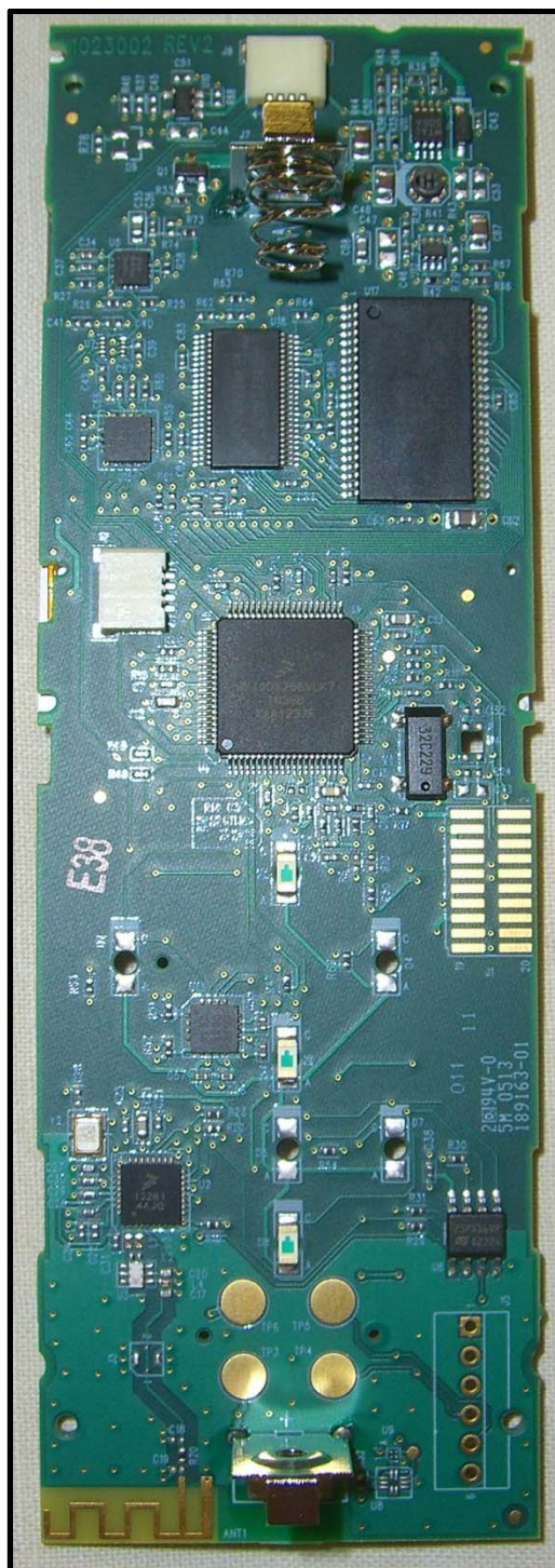
Figure 1 – Rear Side of Circuit Board
