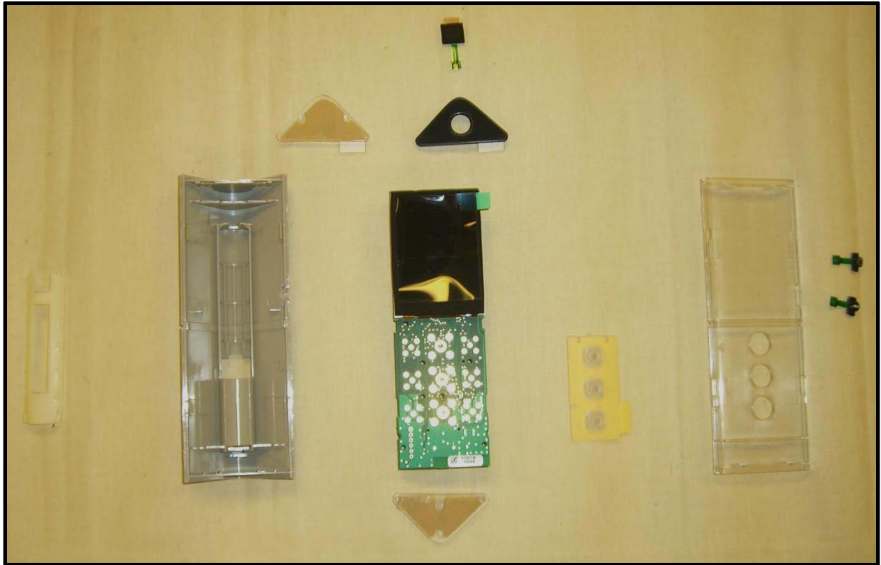
Figure 1 - Assembly Components Front View
