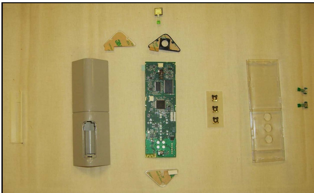
Figure 2 - Assembly Components Rear View
