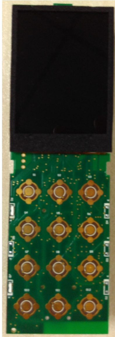
Figure 2 – Front Side of Circuit Board
