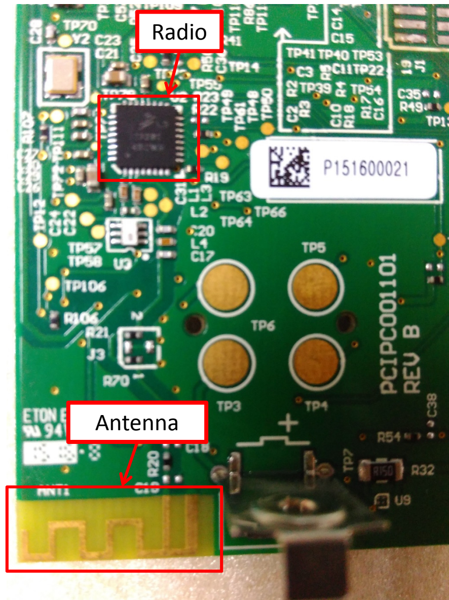
Figure 3 – Detail of antenna and radio on rear side of board
