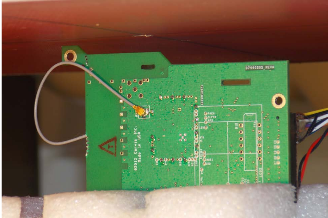
Test Position Internal Antenna Side E 3 mm Gap
