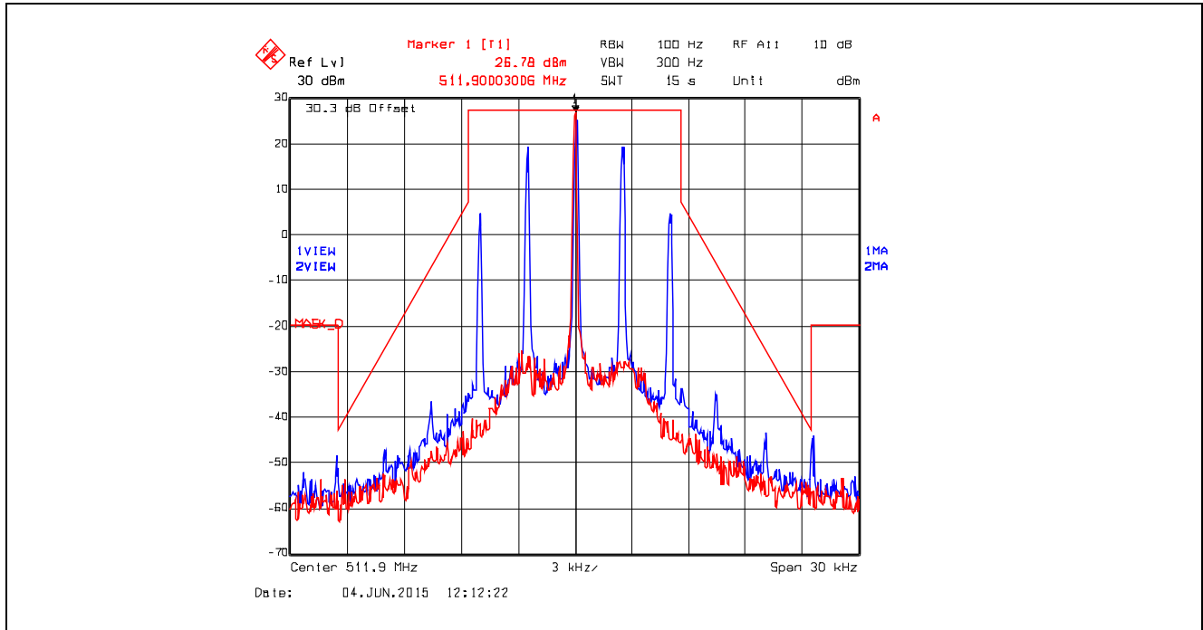
Plot 5.4.4.18. Emission Mask D, Analog, 511.9 MHz, Low Power
