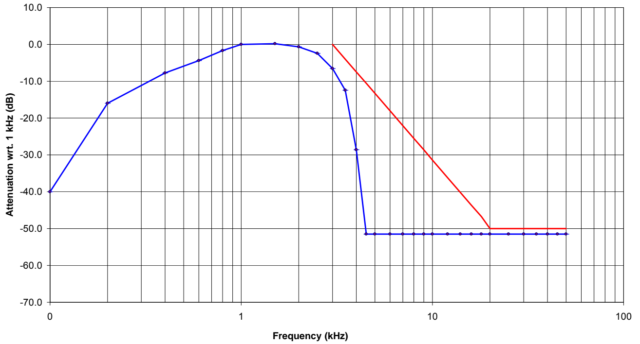
Audio Frequency Response 6.25 kHz Channel Spacing
