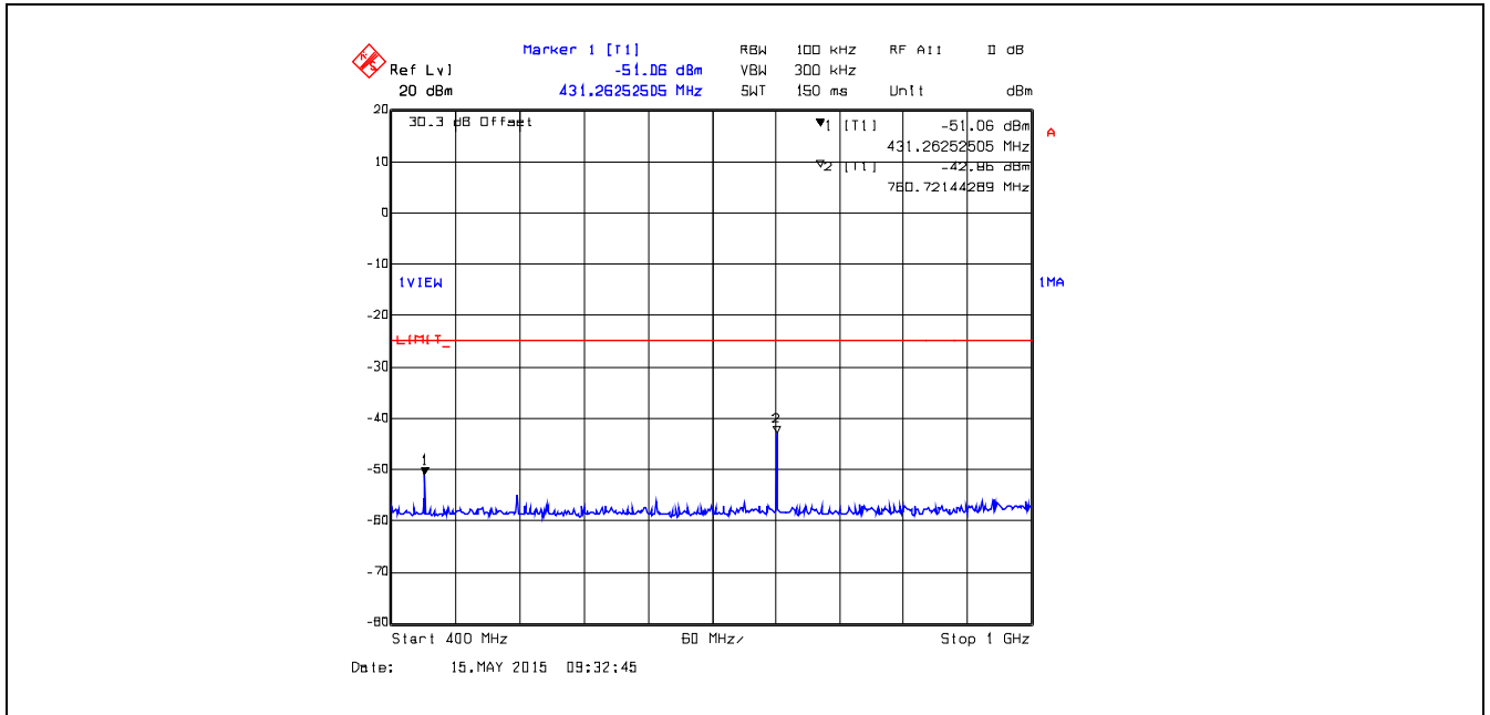
Plot 5.5.4.2. Conducted Transmitter Spurious Emissions, 380.1 MHz, High Power, 400 MHz – 1 GHz
