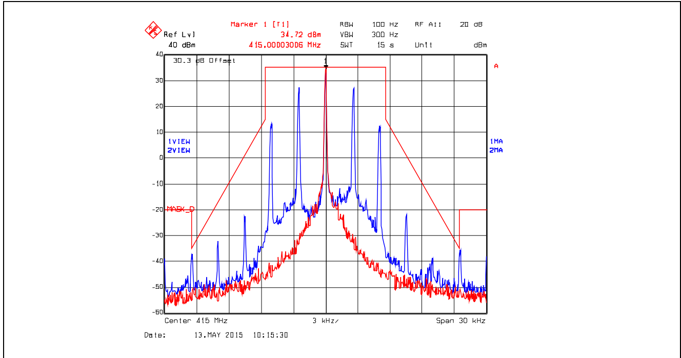
Plot 5.4.4.9. Emission Mask D, Analog, 415.0 MHz, High Power
