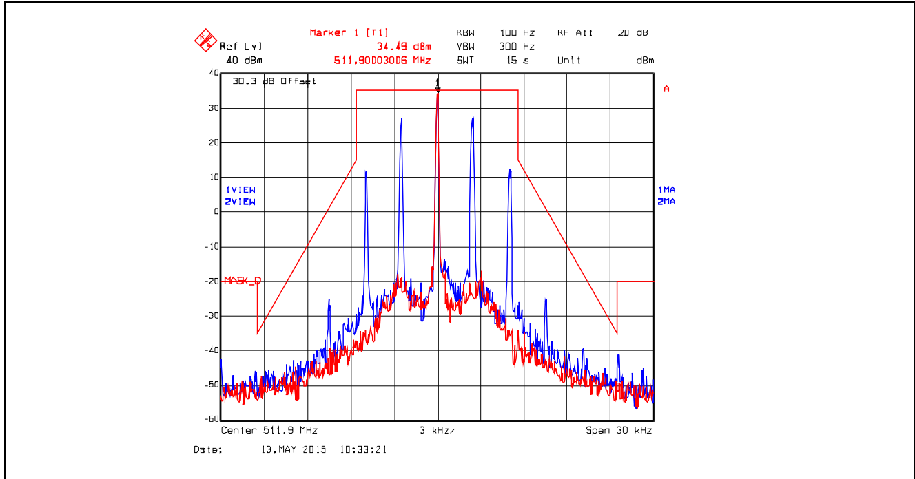
Plot 5.4.4.17. Emission Mask D, Analog, 511.9 MHz, High Power
