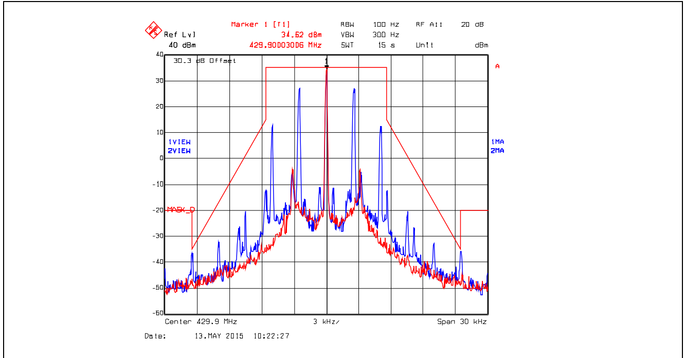
Plot 5.4.4.11. Emission Mask D, Analog, 429.9 MHz, High Power
