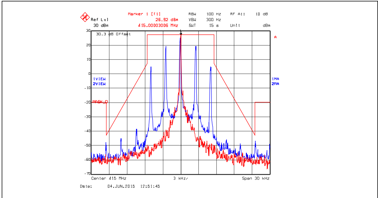
Plot 5.4.4.10. Emission Mask D, Analog, 415.0 MHz, Low Power
