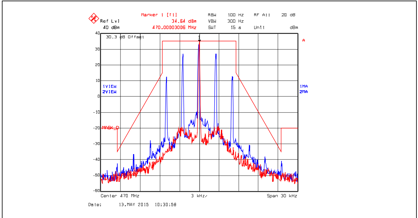
Plot 5.4.4.15. Emission Mask D, Analog, 470.0 MHz, High Power
