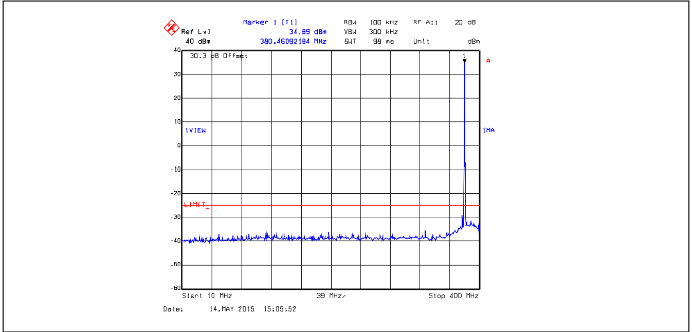
Plot 5.5.4.1. Conducted Transmitter Spurious Emissions, 380.1 MHz, High Power, 10 MHz – 400 MHz
