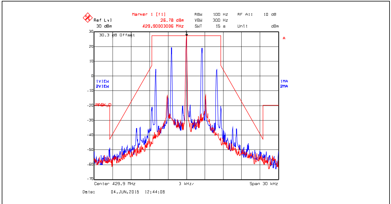
Plot 5.4.4.12. Emission Mask D, Analog, 429.9 MHz, Low Power
