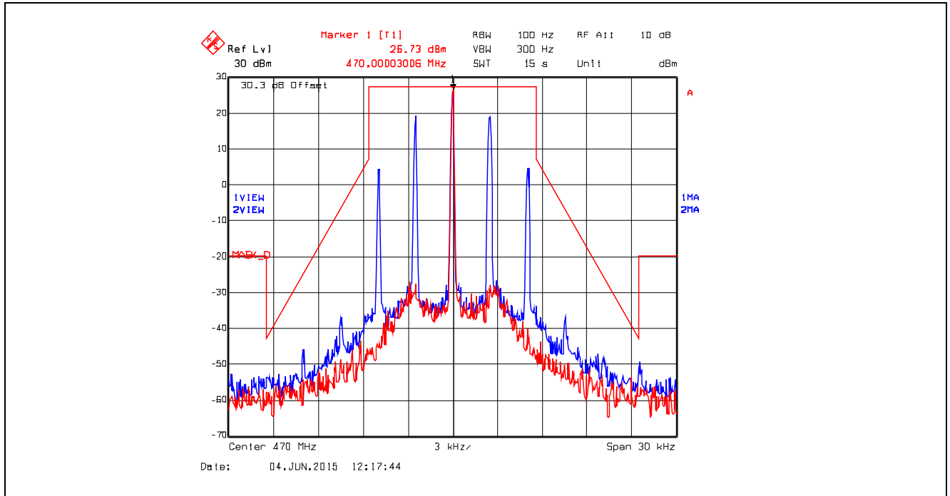
Plot 5.4.4.16. Emission Mask D, Analog, 470.0 MHz, Low Power
