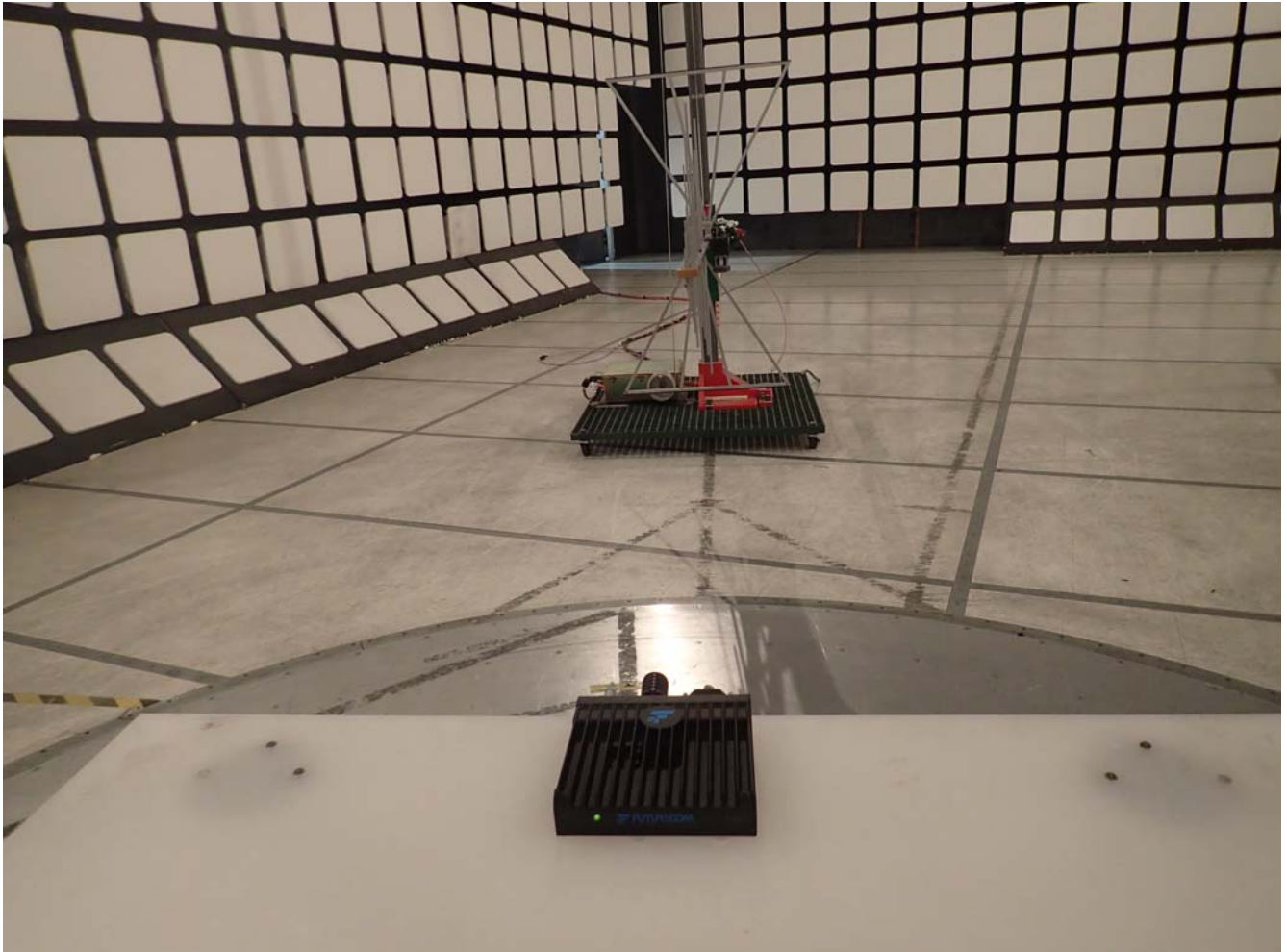
Radiated Emissions at 3 m, 30 - 1000 MHz
