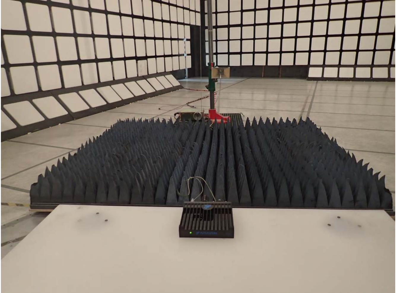
Radiated Emissions at 3 m, Above 1 GHz
