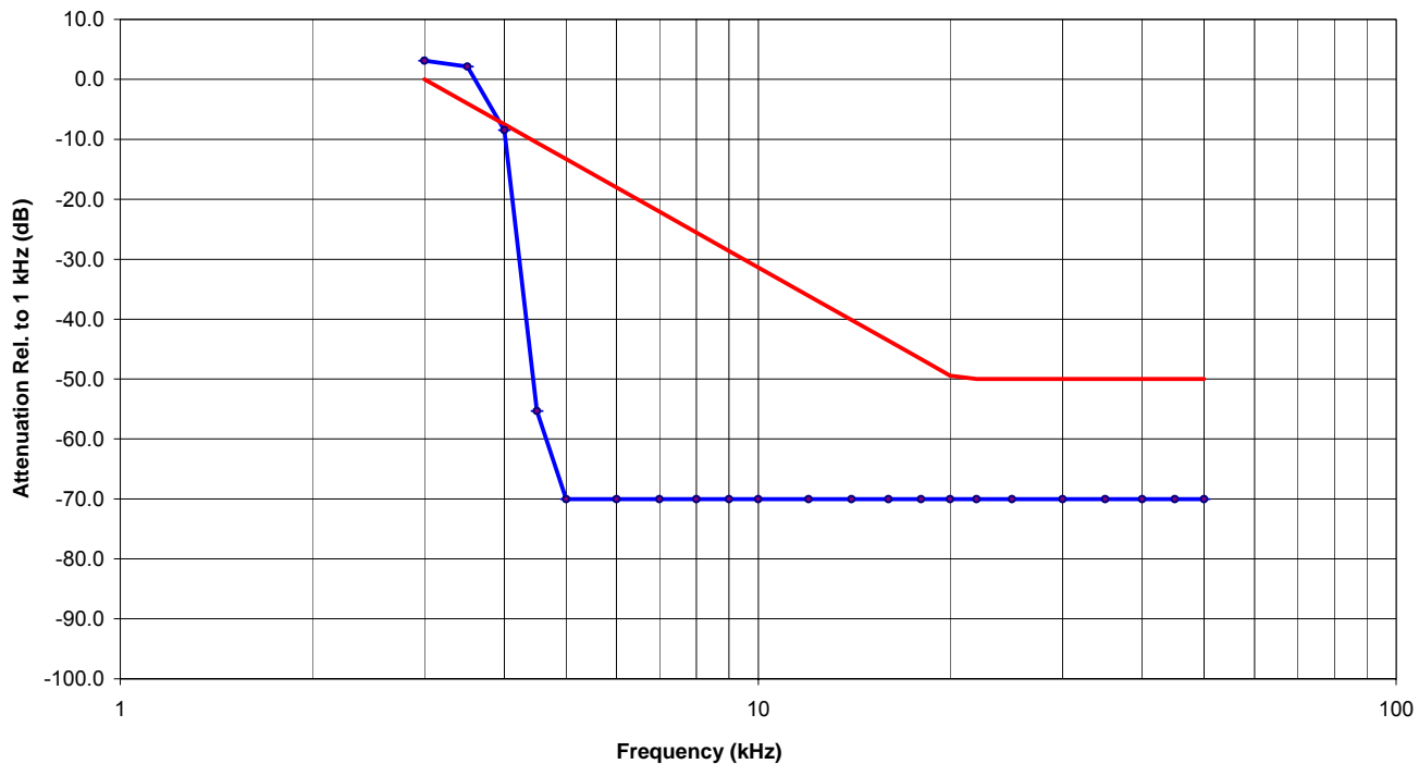
Audio Frequency Response 12.5 kHz Channel Spacing Model: OCR 800
