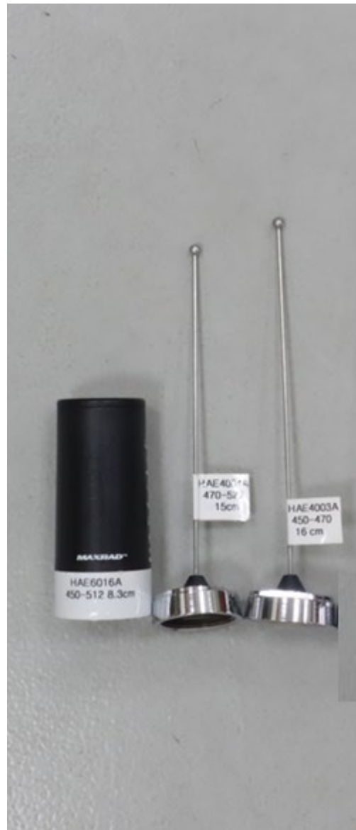
UHF Antenna kit numbers, from left to right; HAE6016A, HAE4004A and HAE4003A
