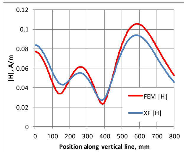
Magnetic field magnitude
