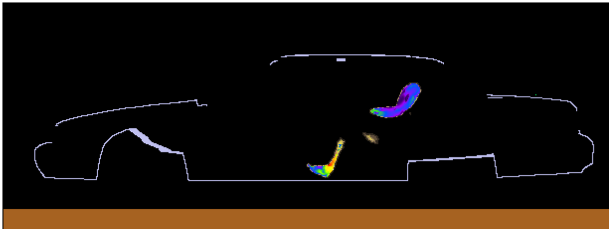
Figure 3. SAR distribution at 167.7 MHz in the passenger back side model produced by the trunk mount HAD4009A antenna. The contour plot is relative to the plane where the peak 1-g average SAR for this exposure condition occurs.
