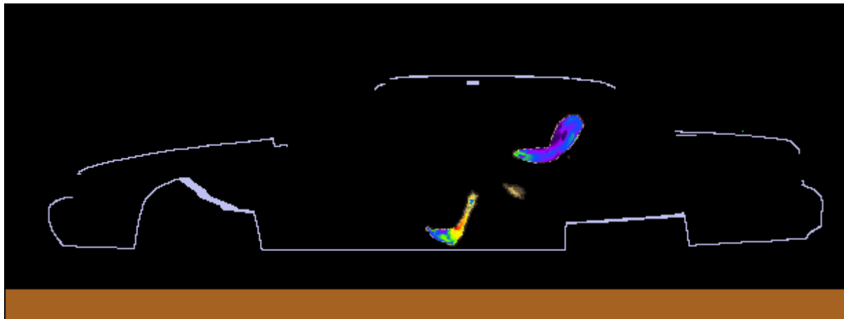
Figure 3. SAR distribution at 167.7 MHz in the passenger back side model produced by the trunk mount HAD4009A antenna. The contour plot is relative to the plane where the peak 1-g average SAR for this exposure condition occurs.
