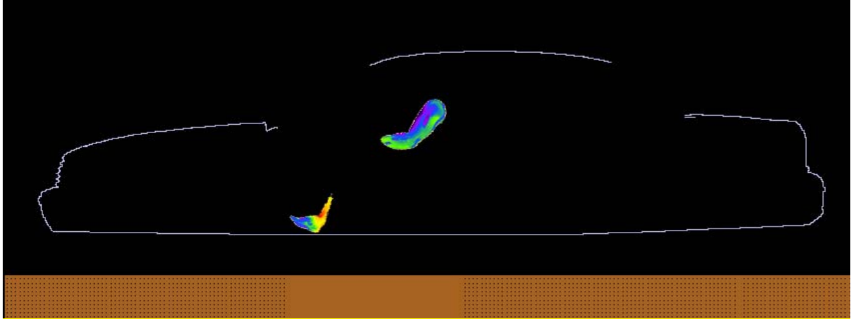
Figure 4. SAR distribution at 150.8 MHz in the driver model produced by the trunk mount HAD4007A antenna. The contour plot is relative to the plane where the peak 1-g average SAR for this exposure condition occurs.
