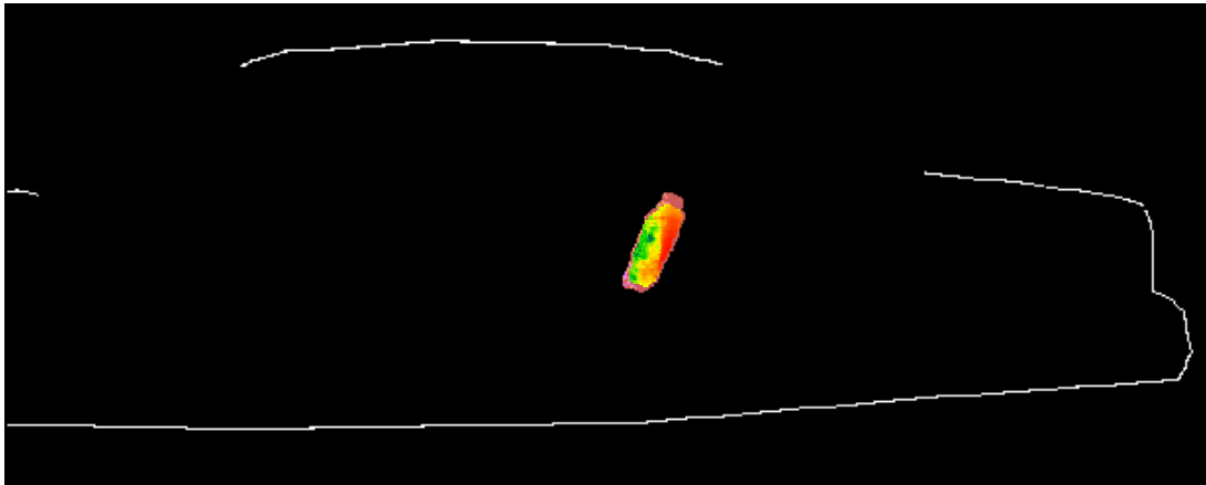
Figure 3. SAR at 512 MHz in the passenger located in the center of the back seat, produced by the trunk-mount HAE4004A antenna. The contour plot in the figure is relative to the plane where the peak 1-g average SAR for this exposure condition occurs.
