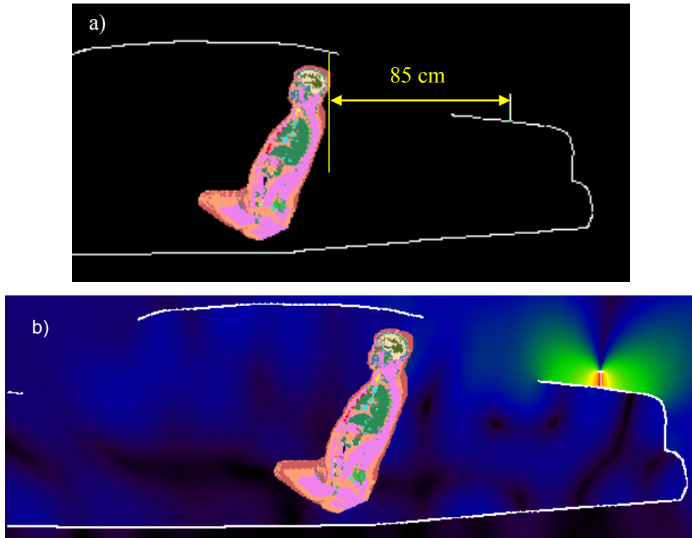
Figure 2: Passenger model exposed to a trunk-mount antenna (8.3 cm) operating at 470 MHz: XFDTD geometry (a) and H-field distribution (b). The antenna is mounted at 85 cm from the passenger.
