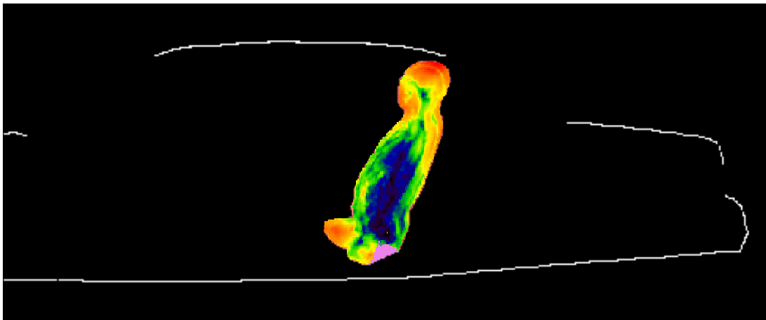
Figure 5. SAR distribution at 425 MHz in the passenger located on the side of the back seat, produced by the roof-mount HAE6013A antenna. The contour plot in the figure is relative to the plane where the peak 1-g average SAR for this exposure condition occurs.
